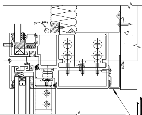
2 TYPICAL TRANSOM DETAIL 6001 CURTAIN WALL
