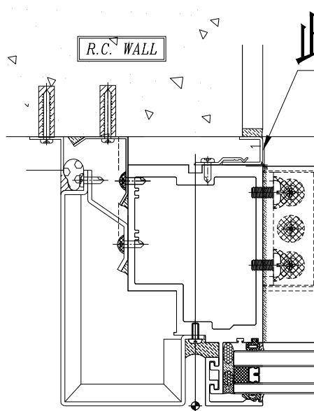
3 TYPICAL MULLION DETAIL 5008 CURTAIN WALL
