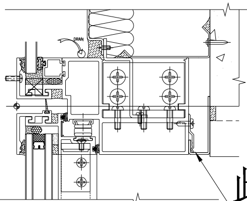
2 TYPICAL TRANSOM DETAIL 6001 CURTAIN WALL
