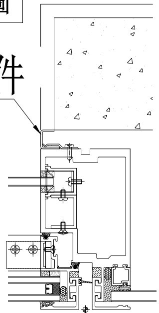
1 TYPICAL MULLION DETAIL CURTAIN WALL 5014
