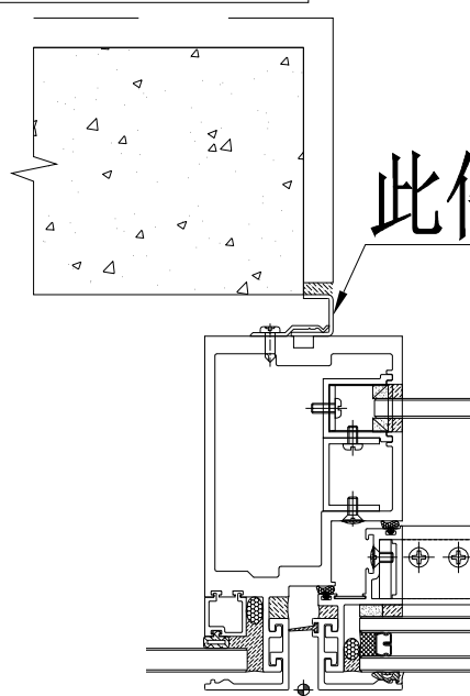
1 TYPICAL MULLION DETAIL 5009 CURTAIN WALL
