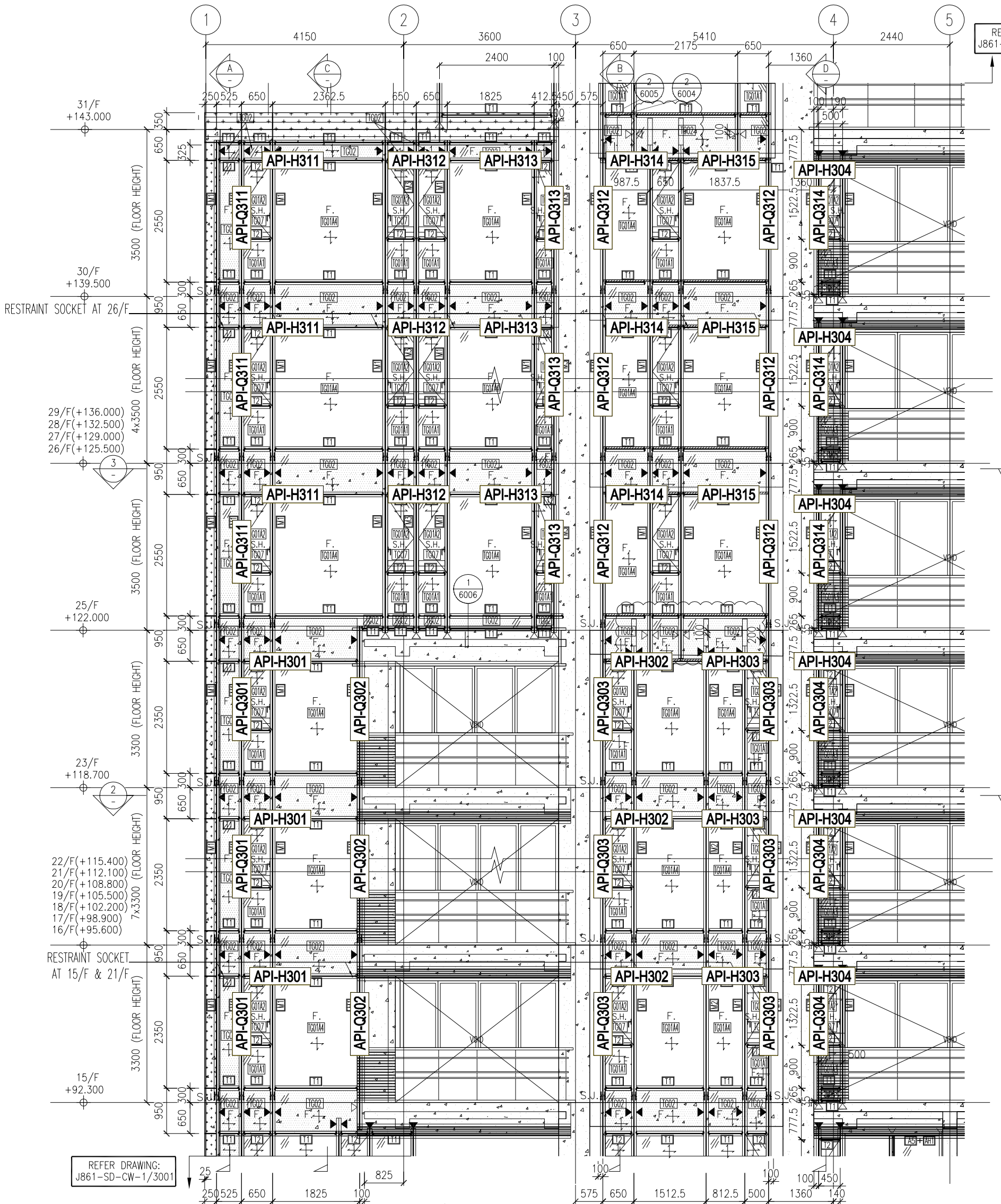
1 PART ELEVATION CURTAIN WALL
