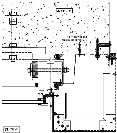
TYPICAL MULLION DETAIL CURTAIN WALL
