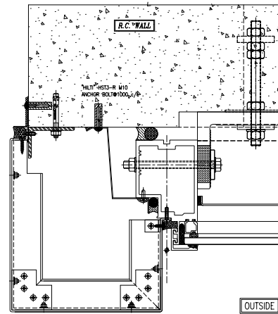
此件 2 TYPICAL MULLION DETAIL 5009 CURTAIN WALL
