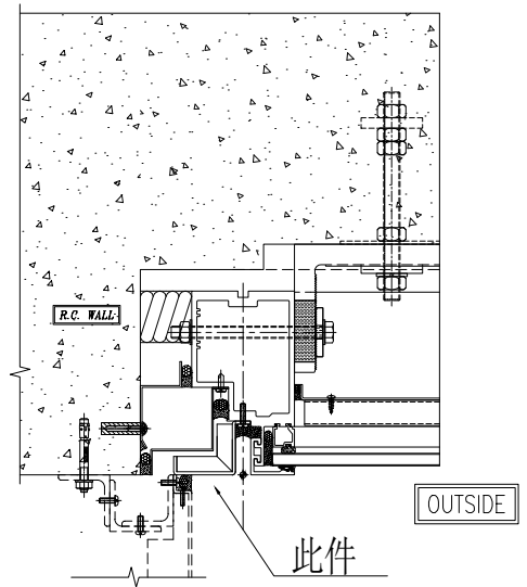
1R TYPICAL MULLION DETAIL 5006 CURTAIN WALL
