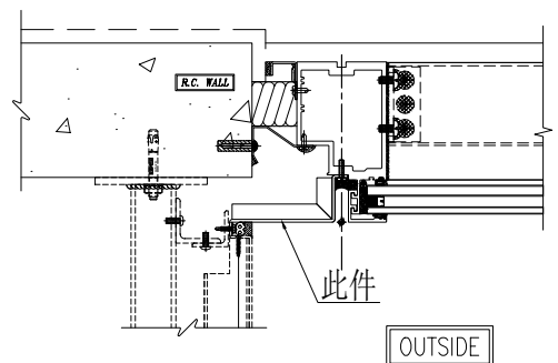
1R 5002 TYPICAL MULLION DETAIL CURTAIN WALL
