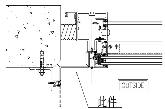
1 5001 TYPICAL MULLION DETAIL CURTAIN WALL
