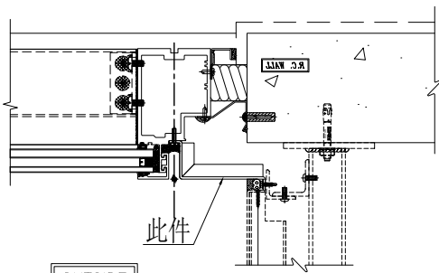
TYPICAL MULLION DETAIL CURTAIN WALL
