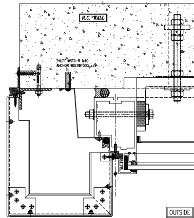
2 5009 TYPICAL MULLION DETAIL CURTAIN WALL
