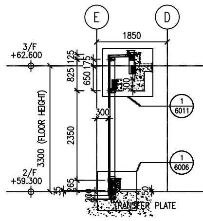
A TYPICAL SECTION CURTAIN WALL
