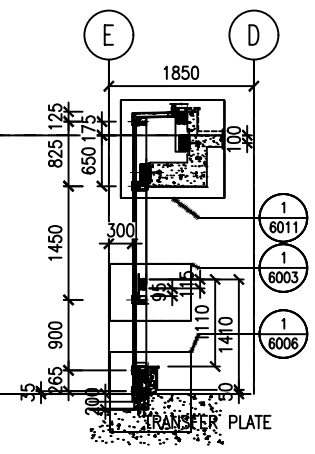
C TYPICAL SECTION CURTAIN WALL
