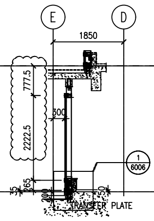
B TYPICAL SECTION CURTAIN WALL
