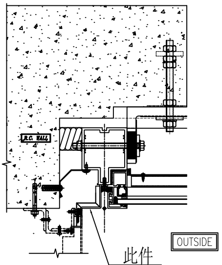
1 TYPICAL MULLION DETAIL 5005 CURTAIN WALL
