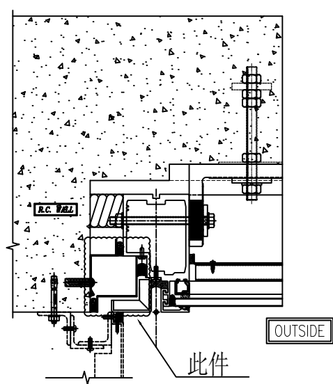
1 TYPICAL MULLION DETAIL 5006 CURTAIN WALL
