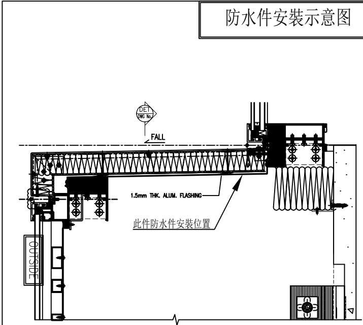
1 TYPICAL TRANSOM DETAIL 6011 CURTAIN WALL
