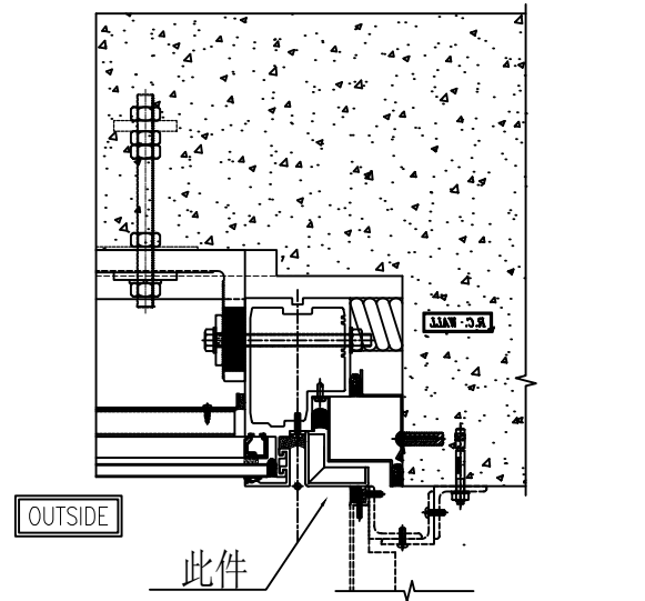
TYPICAL MULLION DETAIL CURTAIN WALL 1R 5006
