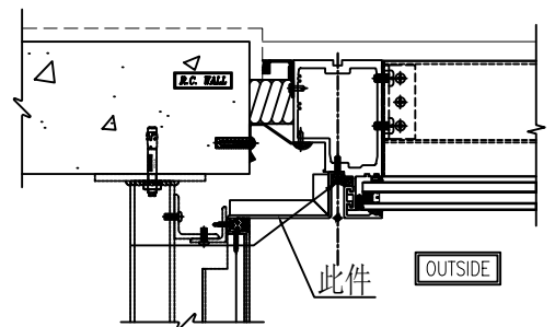
1 5002 TYPICAL MULLION DETAIL CURTAIN WALL
