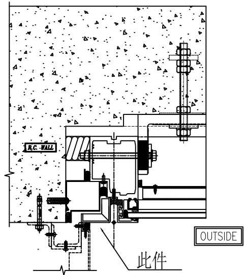
1 TYPICAL MULLION DETAIL 5006 CURTAIN WALL
