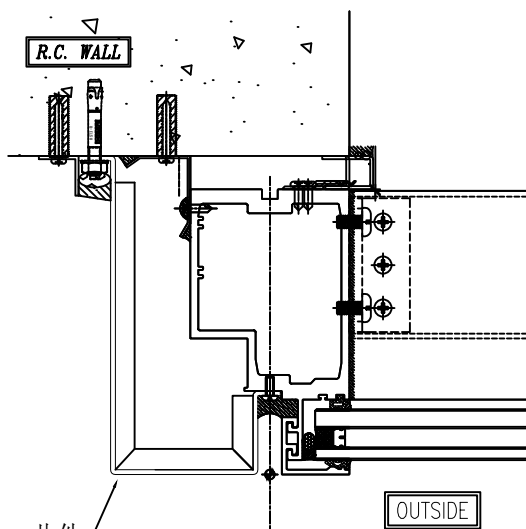
3 TYPICAL MULLION DETAIL 5008 CURTAIN WALL
