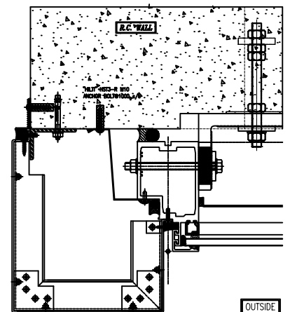
此件 2 TYPICAL MULLION DETAIL 5009 CURTAIN WALL
