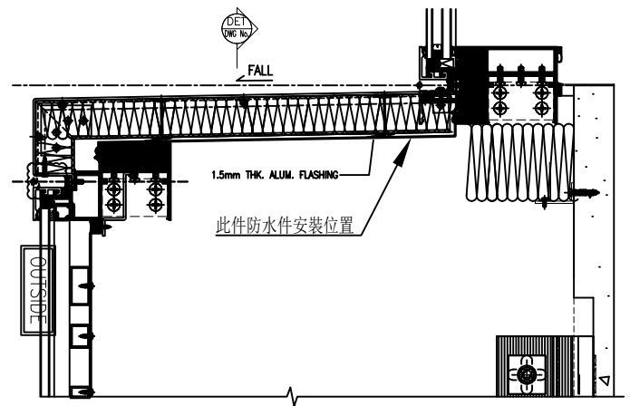
1 TYPICAL TRANSOM DETAIL 6011 CURTAIN WALL
