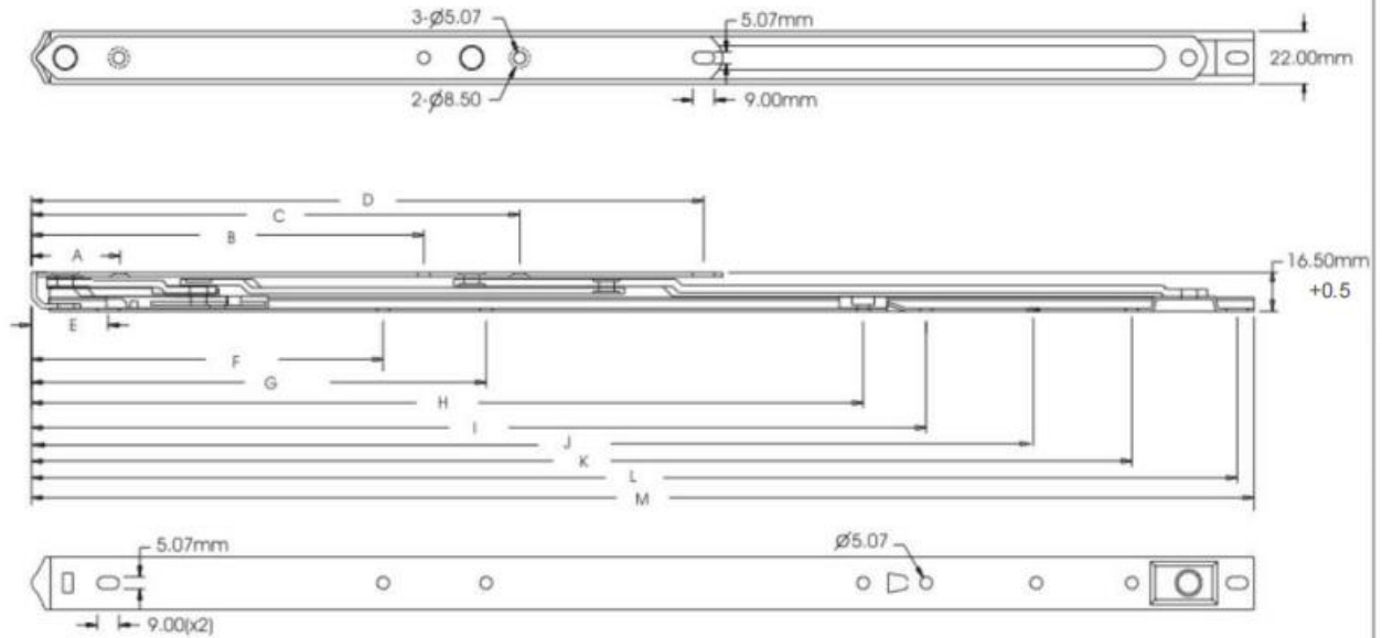
尺寸 MEASUREMENTS (mm)
