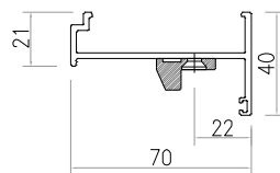
SECTION C-C
