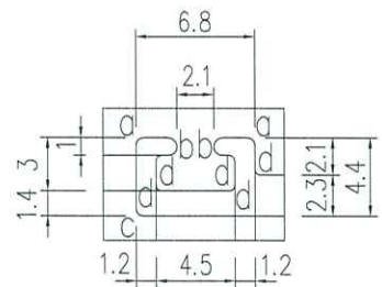
detail E scale 2:1
