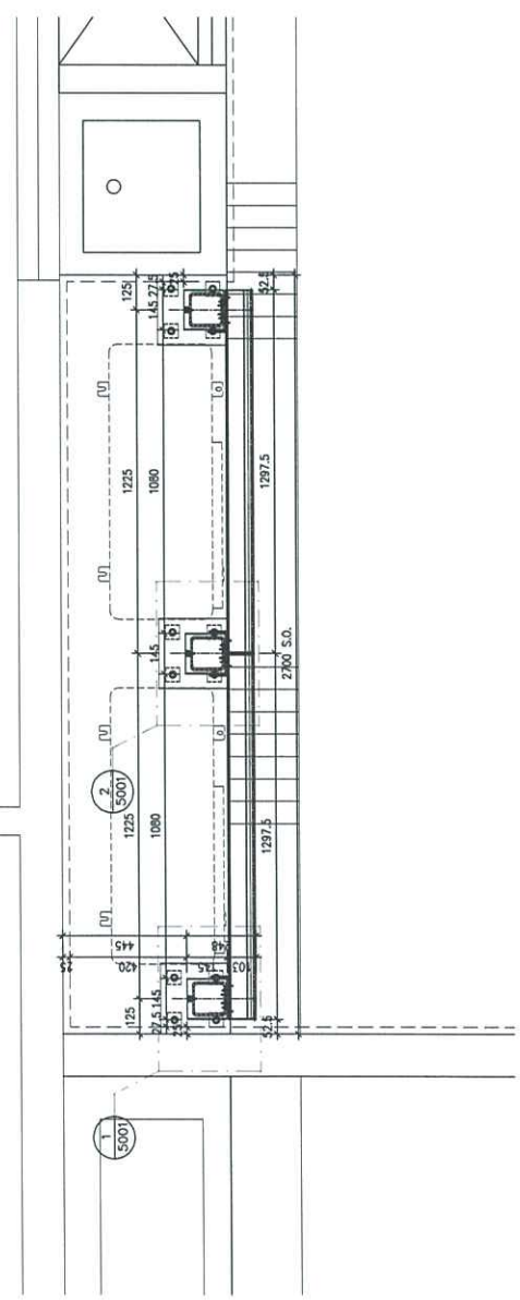
PART PLAN
