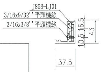
SECTION C-C
