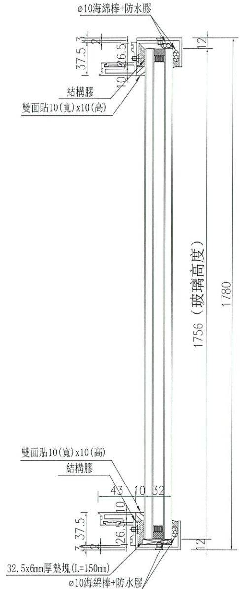
SECTION B-B
