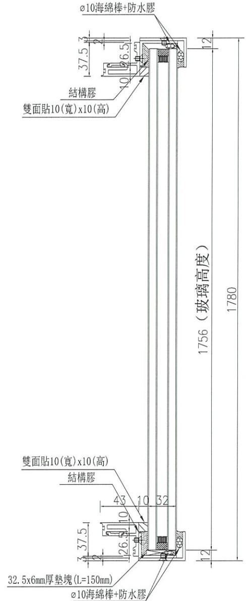
SECTION B-B
