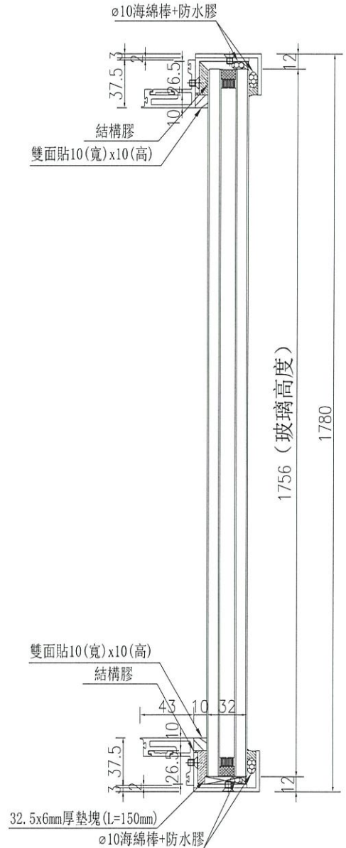
SECTION B-B
