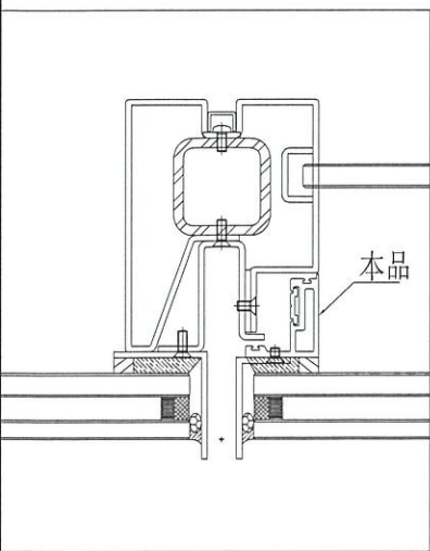
SECTION C-C
