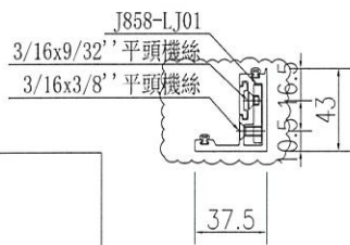
SECTION C-C
