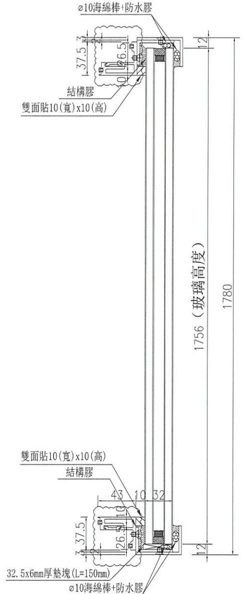
SECTION B-B
