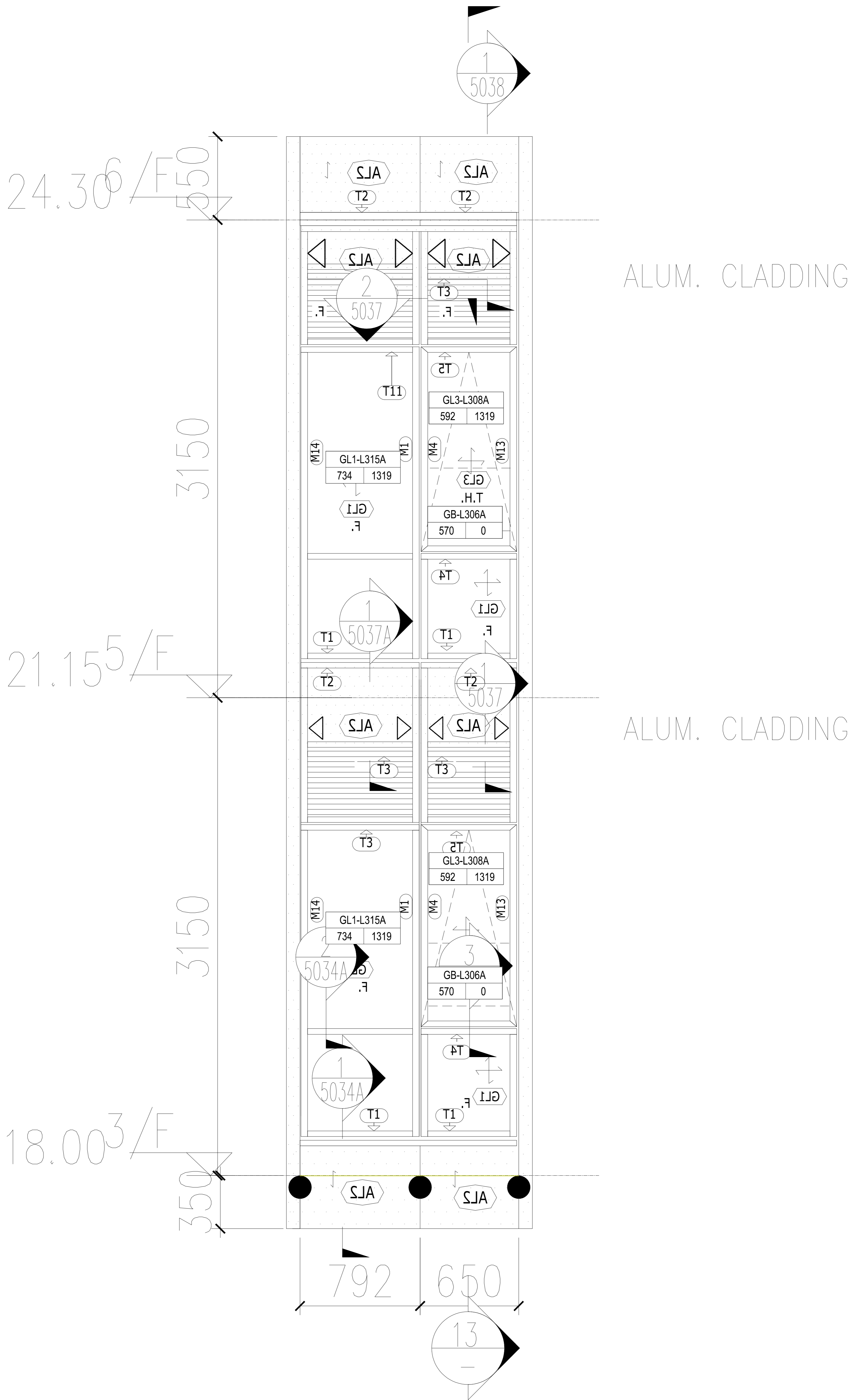
10 3018 TOWER L - PART ELEVATION 1:50
