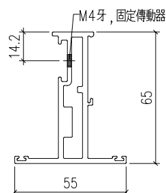
剖圖C-C
