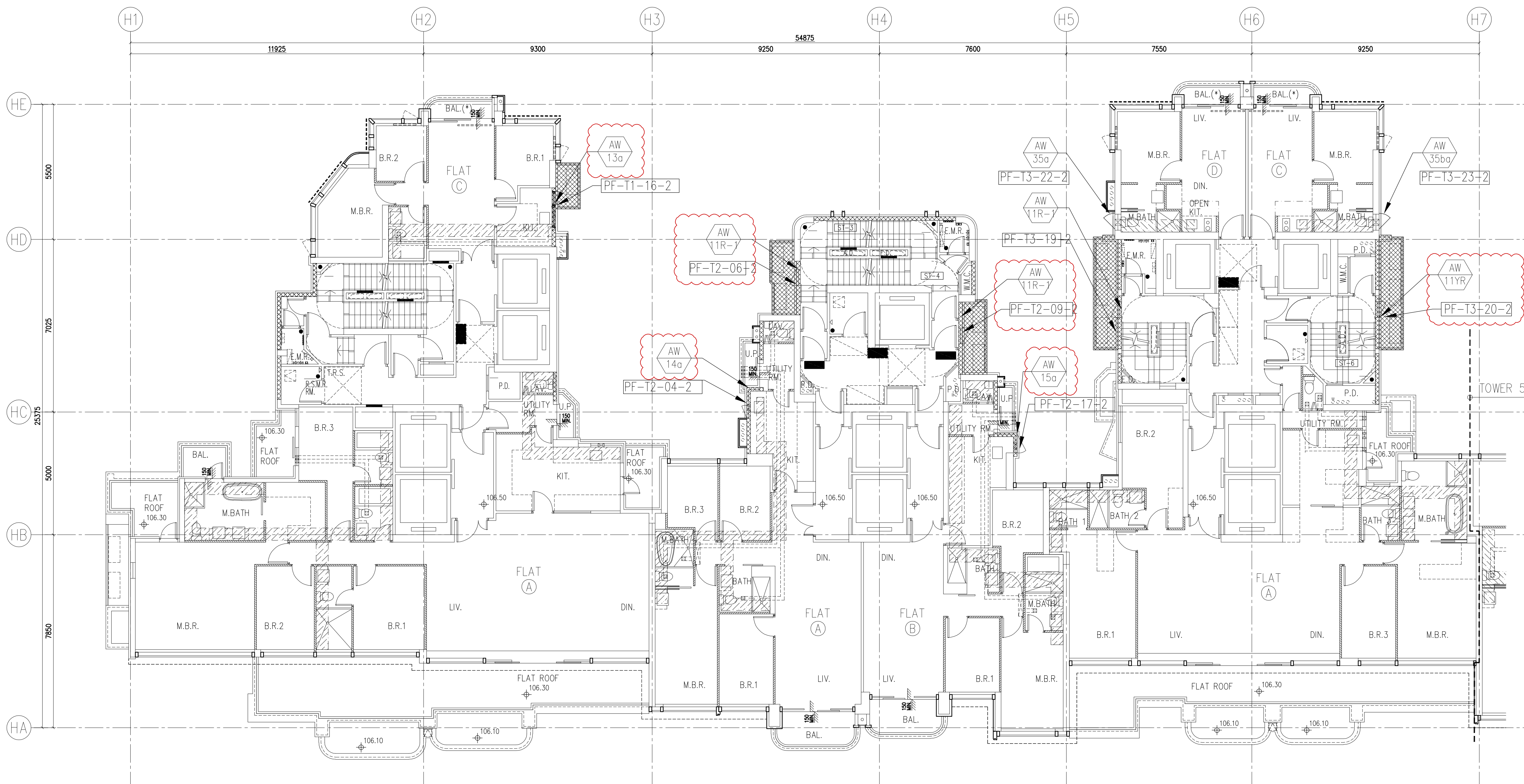
TOWER 1 33/F PLAN
