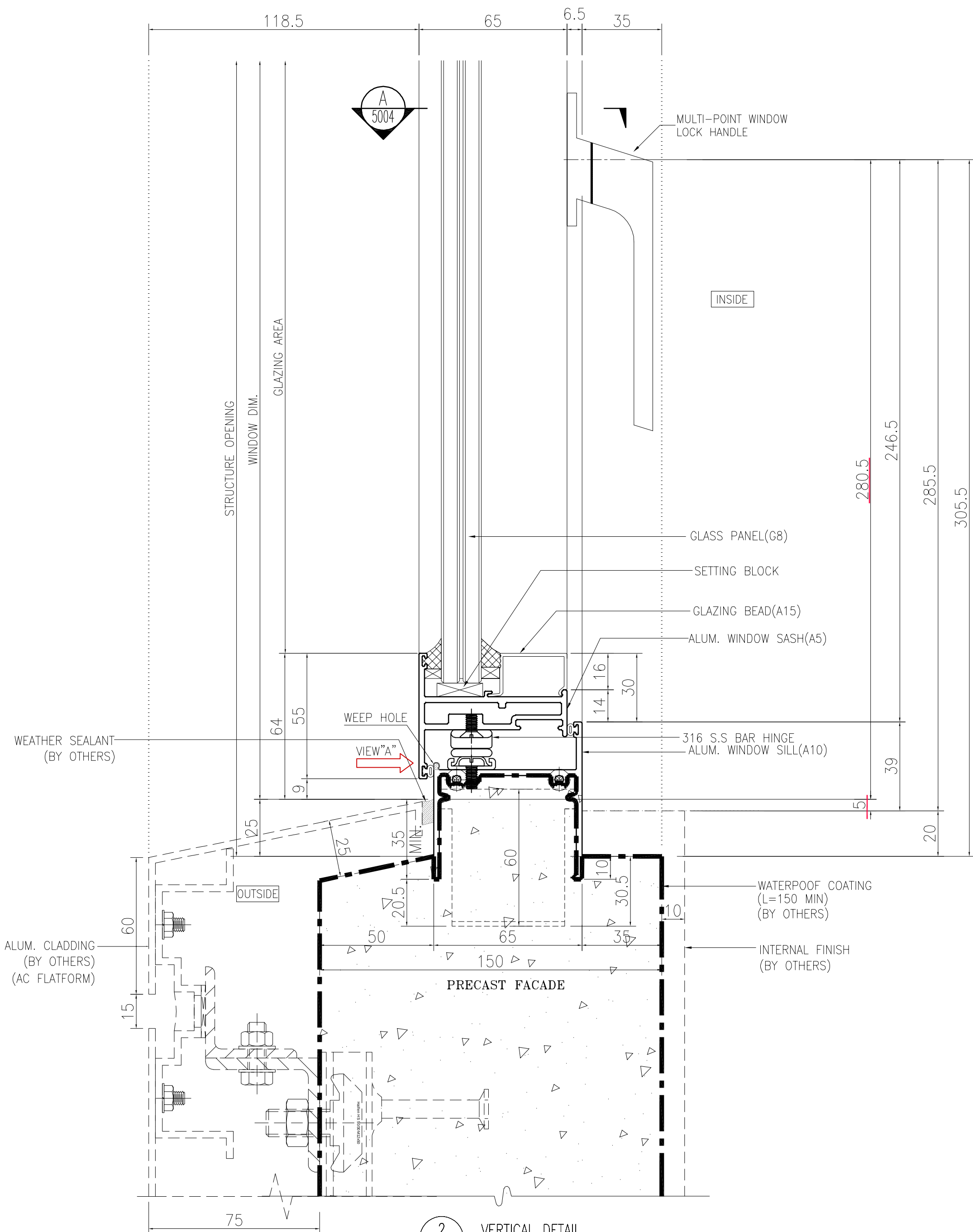
2 6001 VERTICAL DETAIL Openable Window
