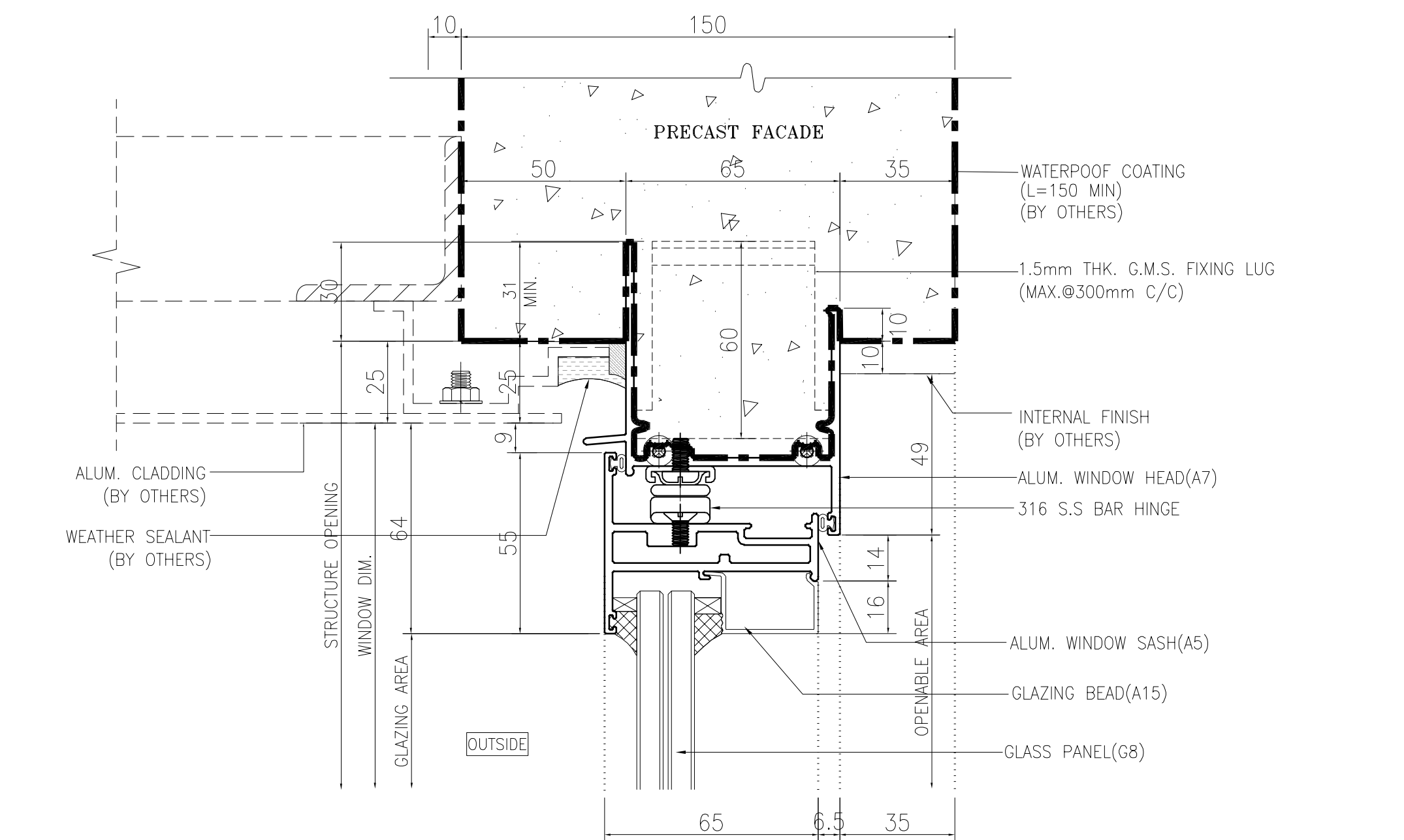
1 6001 VERTICAL DETAIL Openable Window
