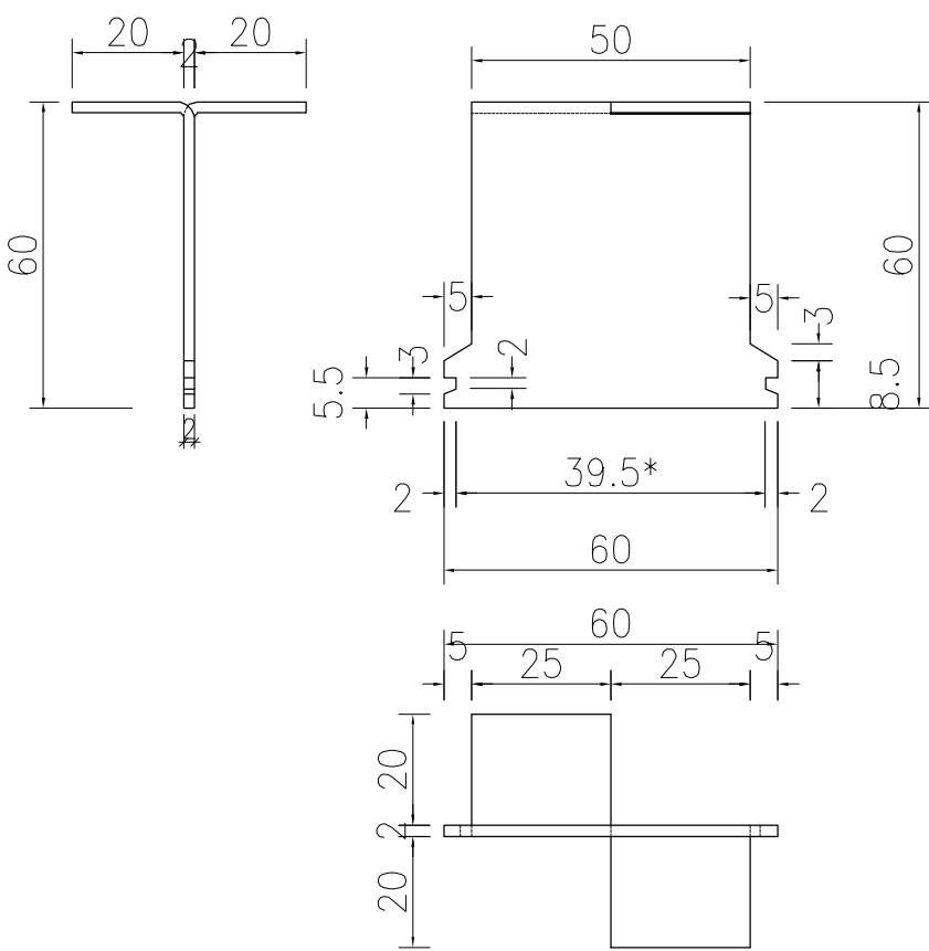
03 -- TYPICAL G.M.S. FIXING LUG DETAIL 1:2
