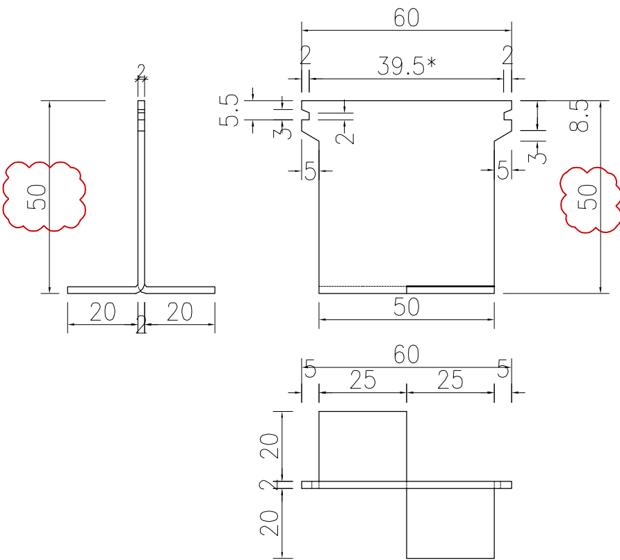
03a -- TYPICAL G.M.S. FIXING LUG DETAIL 1:2
