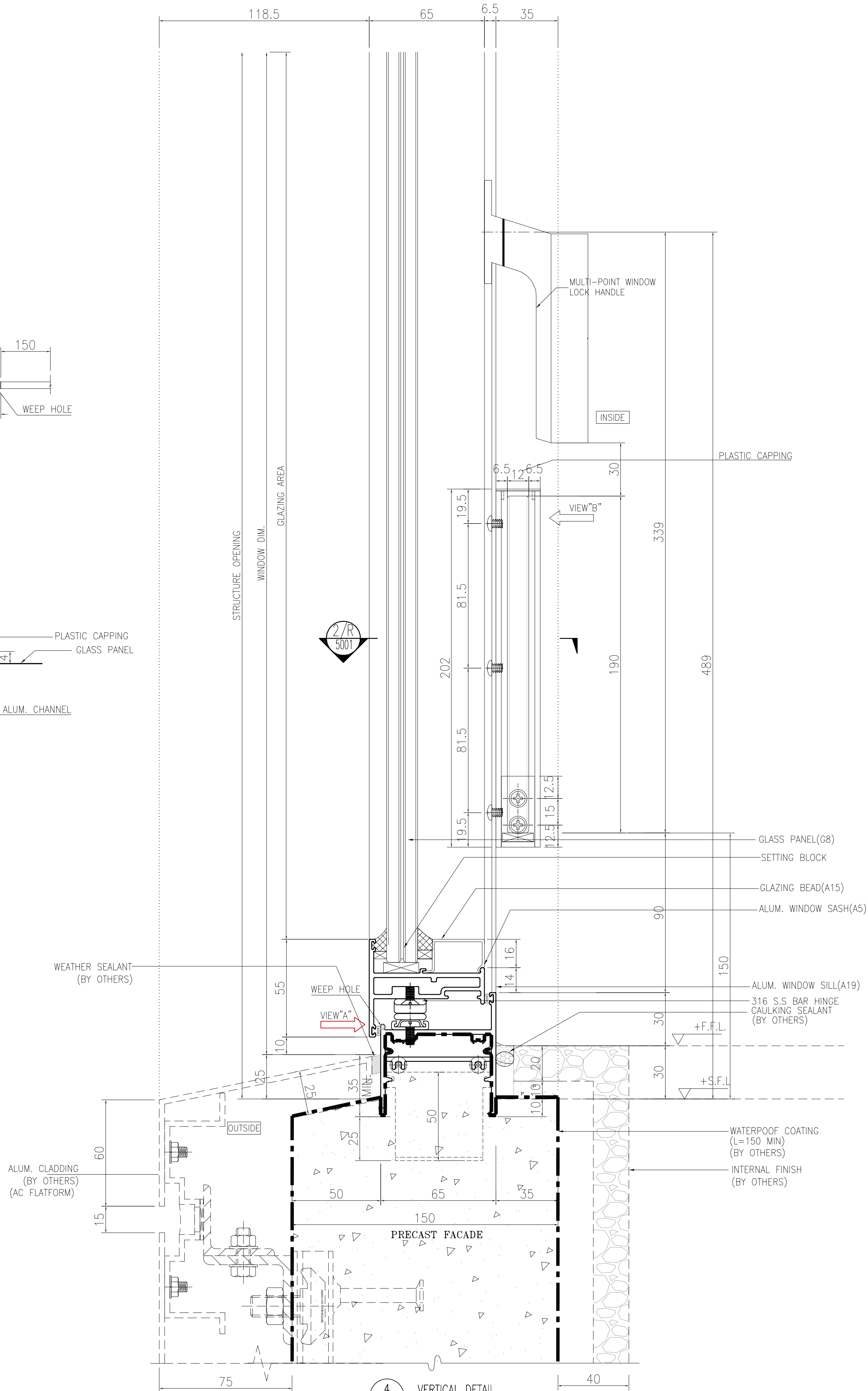
4 6001 VERTICAL DETAIL Openable Window
