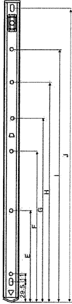
客戶安裝尺寸 The Installation Dimensions(mm)
