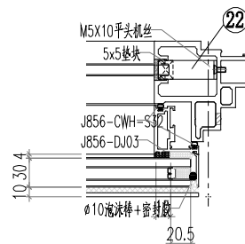
VIEW E
