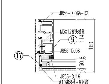
VIEW E
