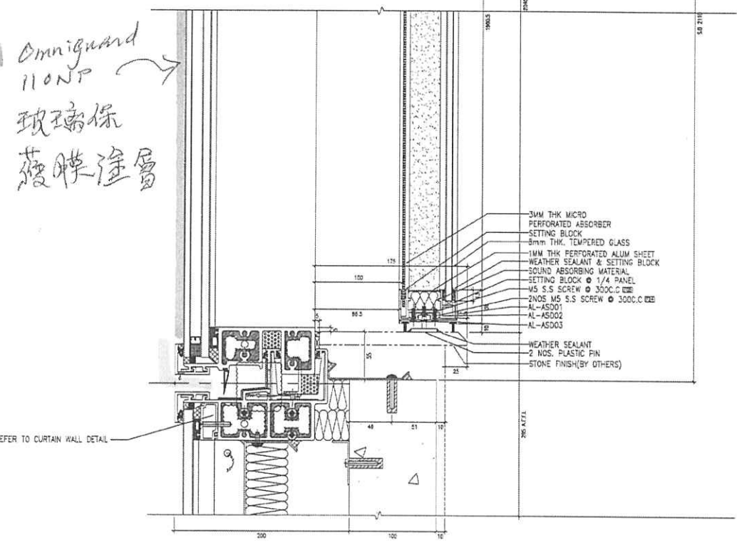
SECTION DETAIL ACUSTIC SCREEN FIN1
