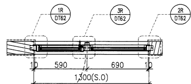
PART PLAN A1
