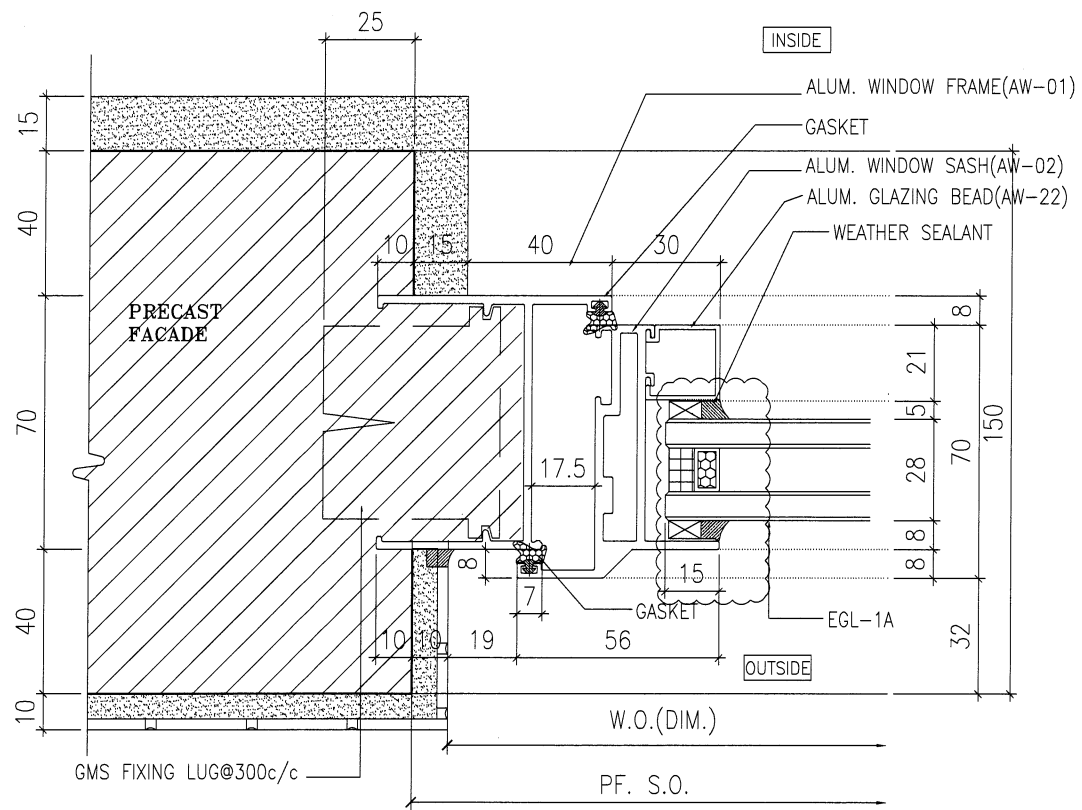
1 HORIZONTAL DETAIL SCALE 1:2
