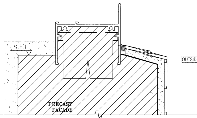
2 HORIZONTAL DETAIL SCALE 1:2
