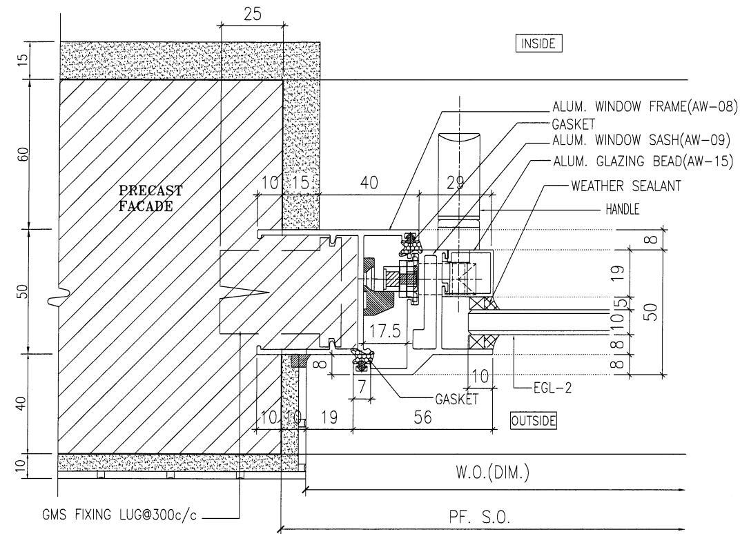
1 HORIZONTAL DETAIL SCALE 1:2
