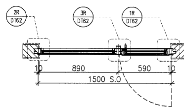
A1 PART PLAN
