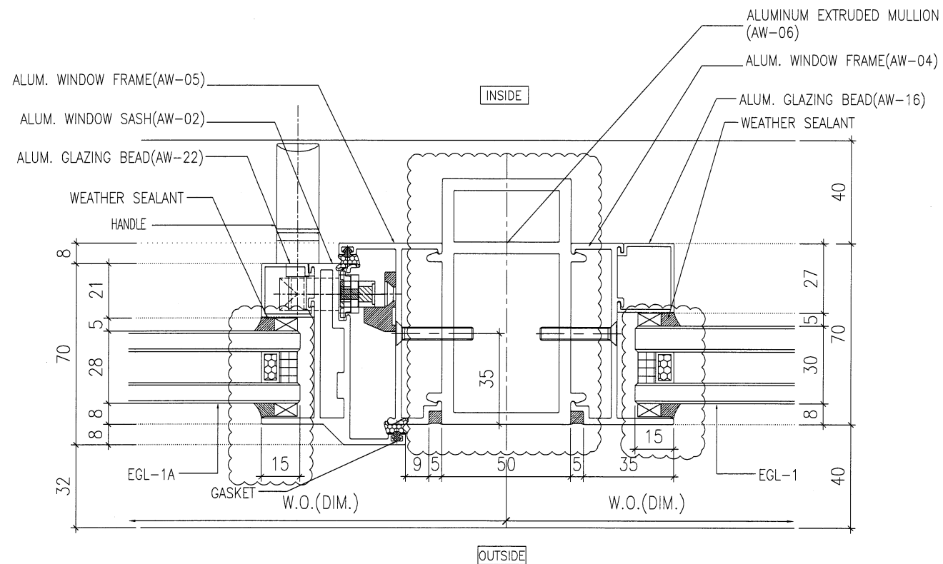
3 HORIZONTAL DETAIL SCALE 1:2
