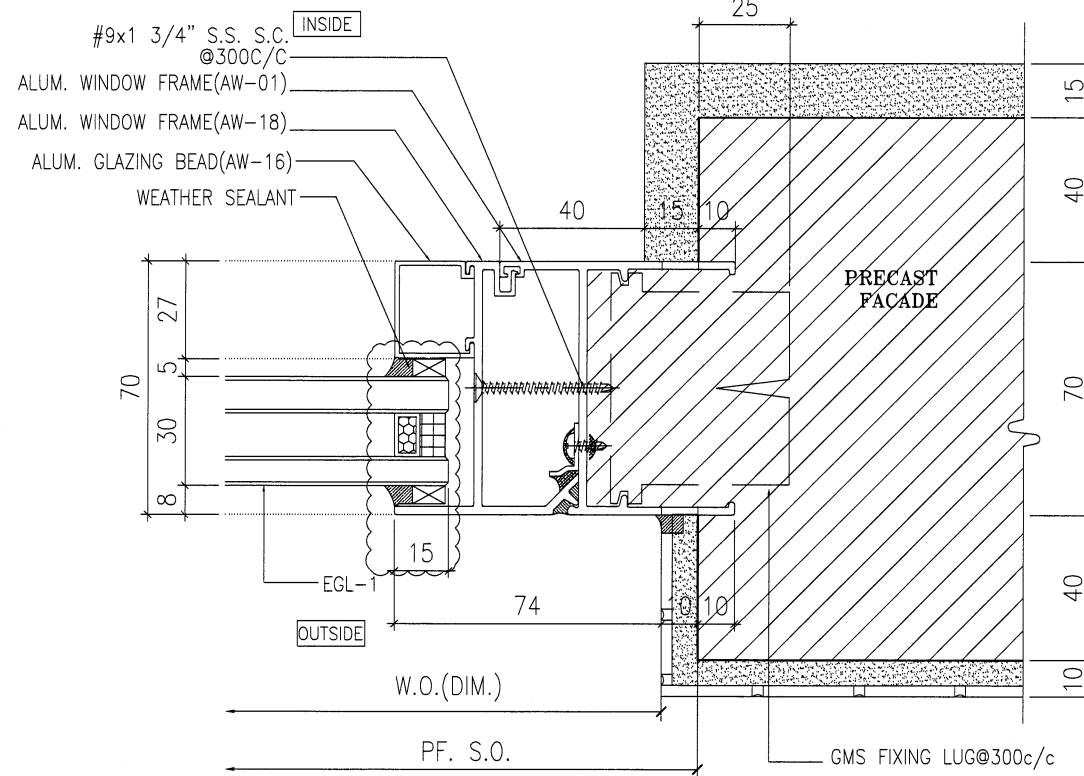
4 HORIZONTAL DETAIL SCALE 1:2
