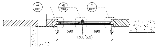
A2 PART PLAN
