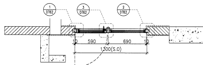
A1 PART PLAN
