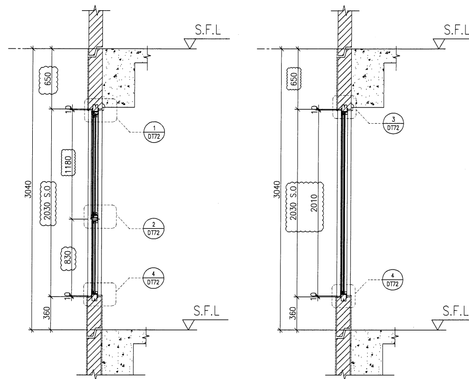
X PART SECTION
