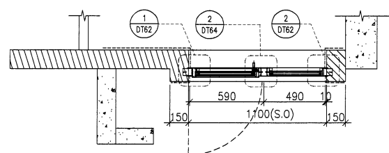
A1 PART PLAN
