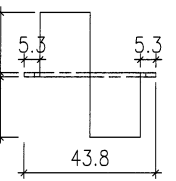
3 HORIZONTAL DETAIL SCALE 1:2
