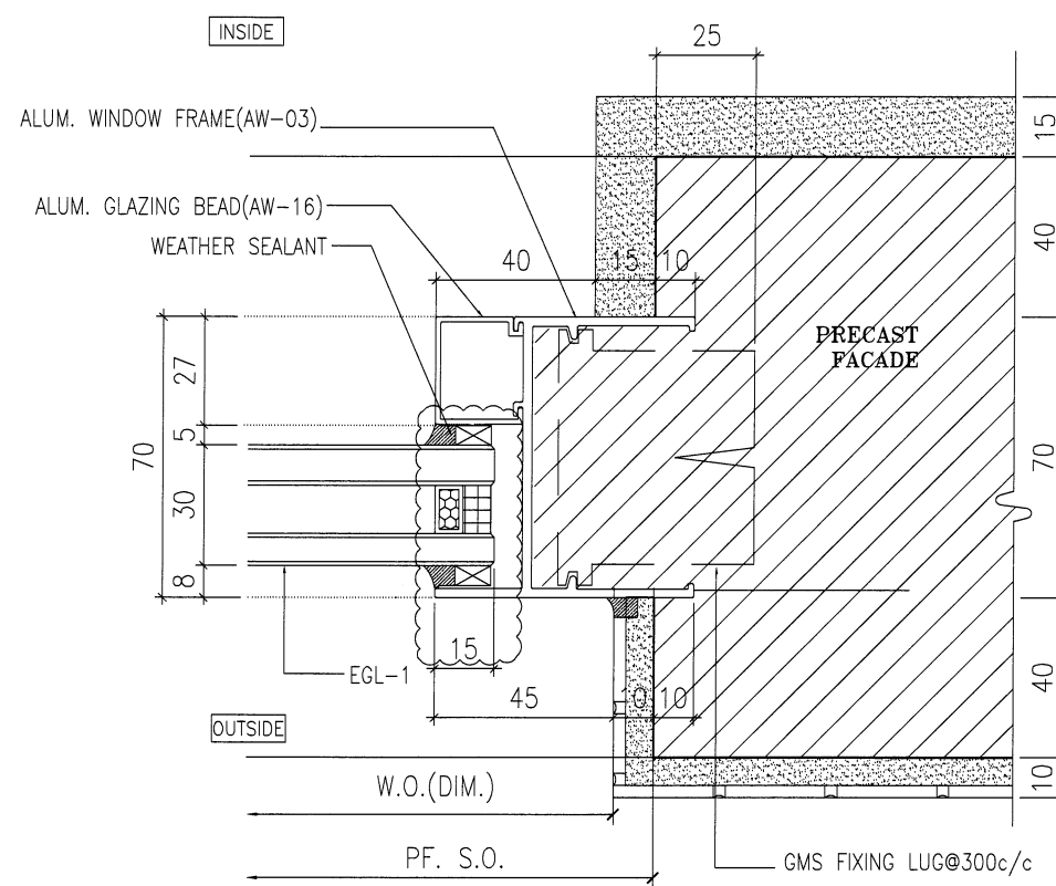
2 HORIZONTAL DETAIL SCALE 1:2
