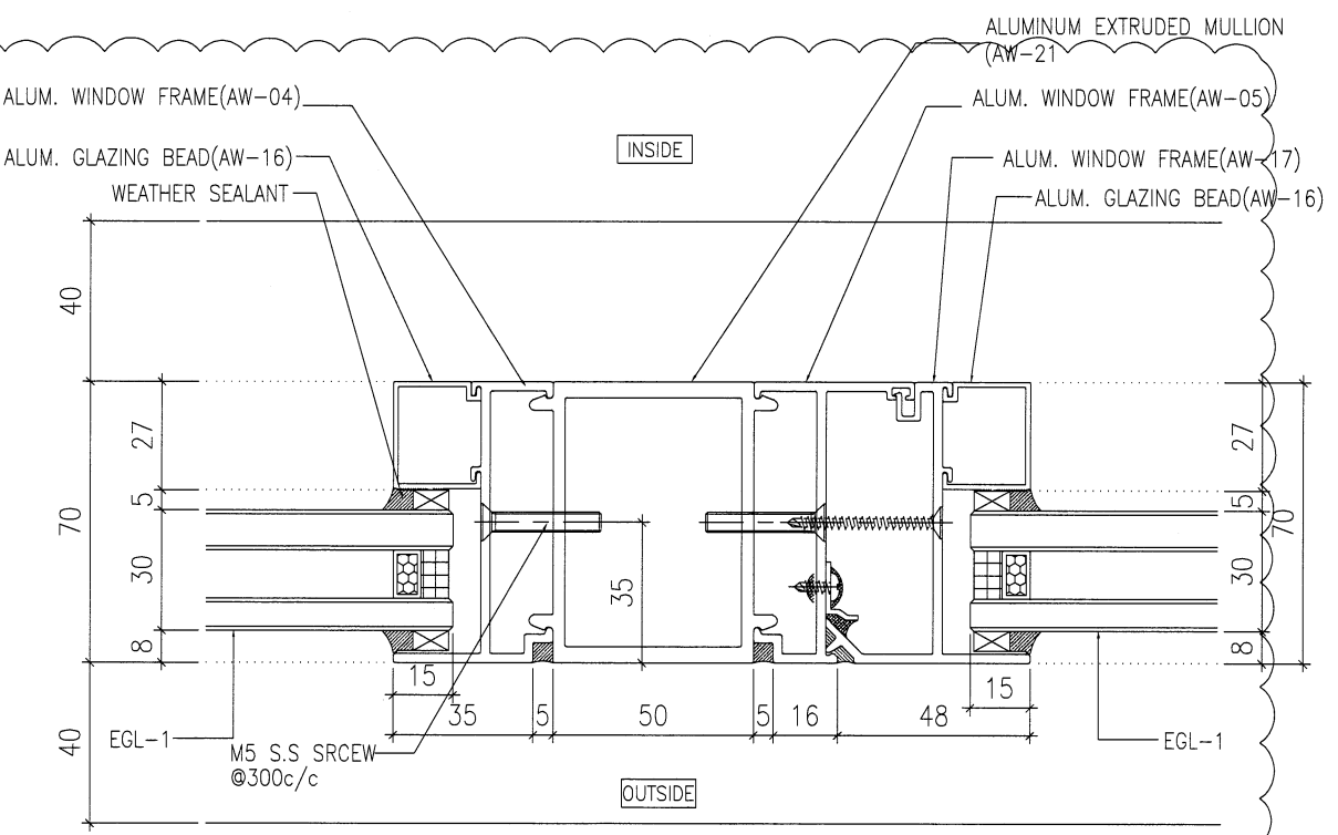
3 HORIZONTAL DETAIL SCALE 1:2
