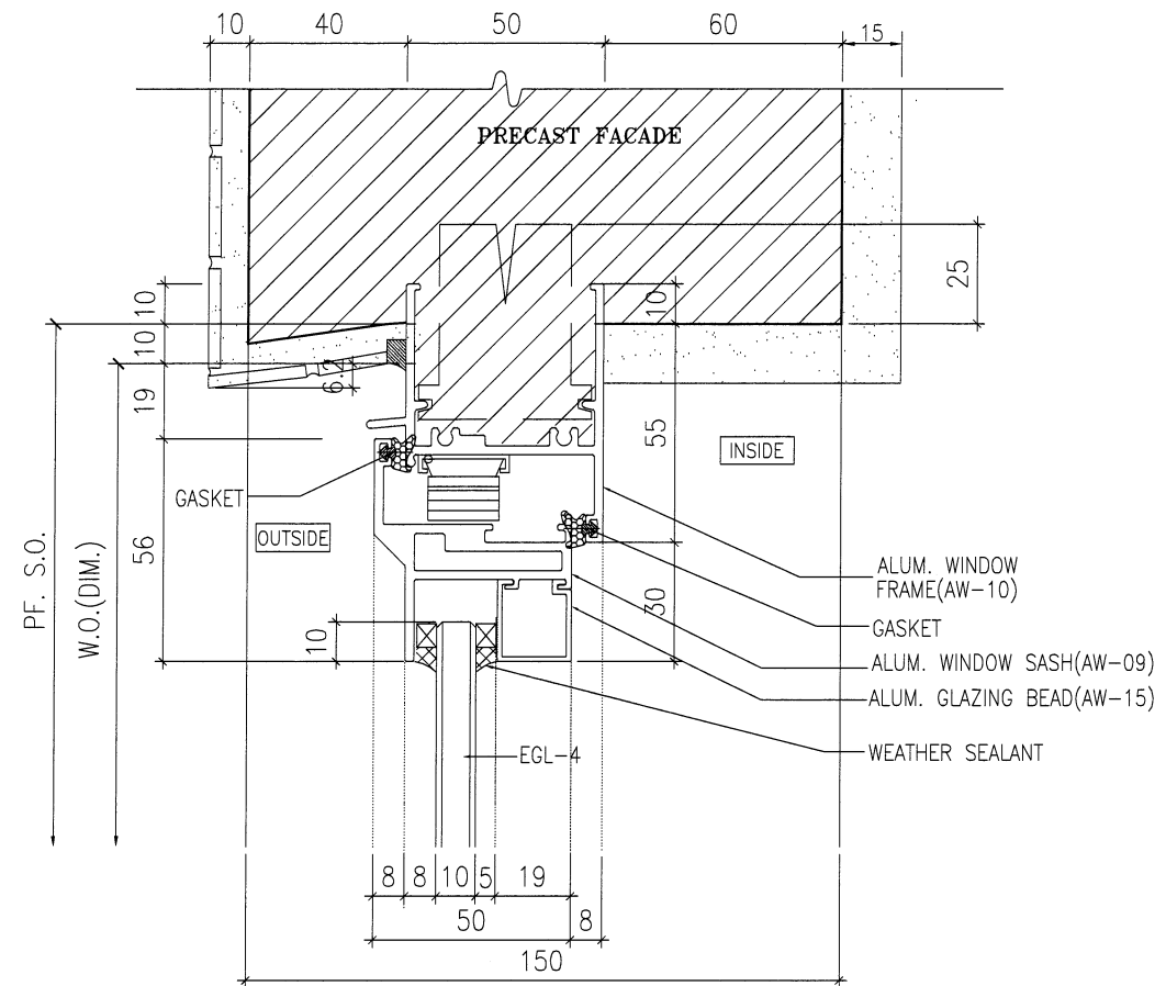
1 HORIZONTAL DETAIL SCALE 1:2 150
