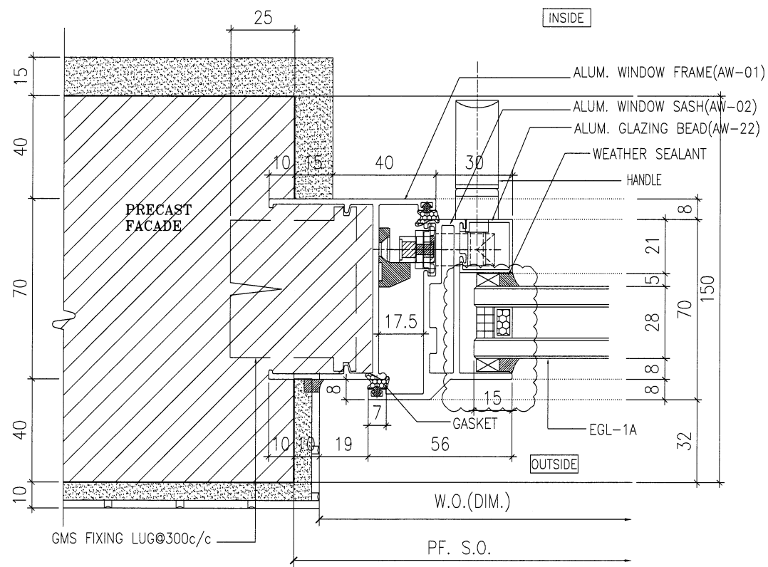
3 HORIZONTAL DETAIL SCALE 1:2
