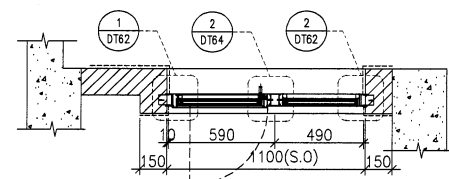
A1 PART PLAN
