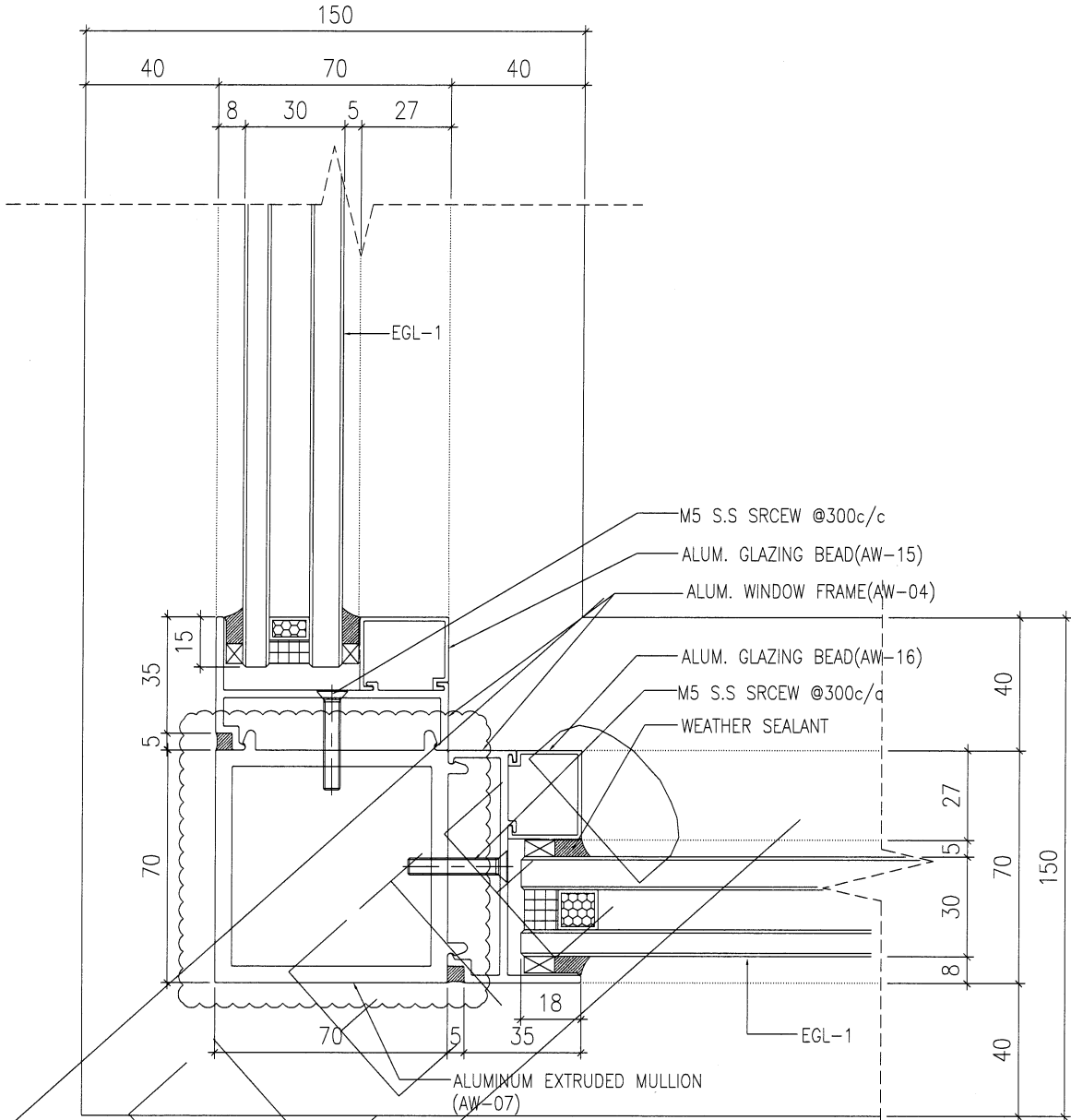
2 HORIZONTAL DETAIL SCALE 1:2
