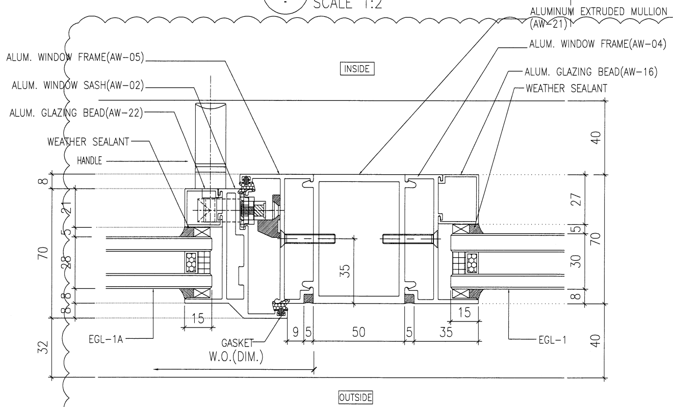
2 HORIZONTAL DETAIL SCALE 1:2
