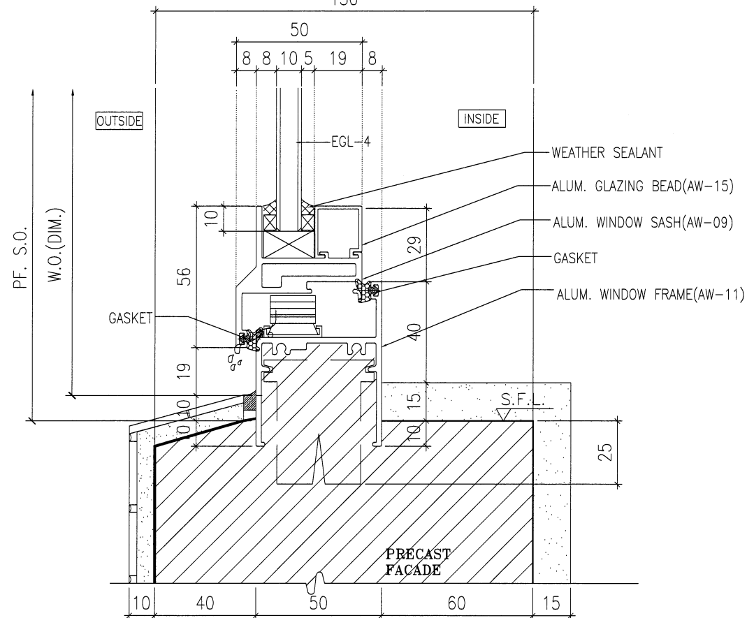
2 HORIZONTAL DETAIL SCALE 1:2 150
