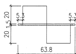
2 HORIZONTAL DETAIL SCALE 1:2
