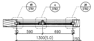
PART PLAN A2
