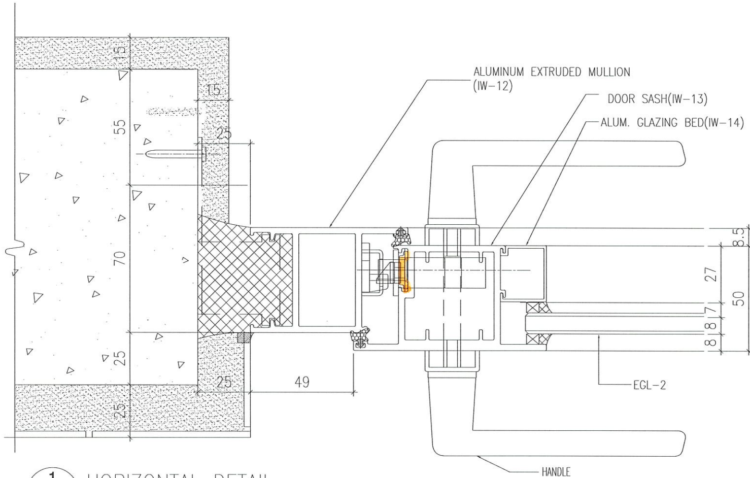
1 HORIZONTAL DETAIL SCALE 1:2
