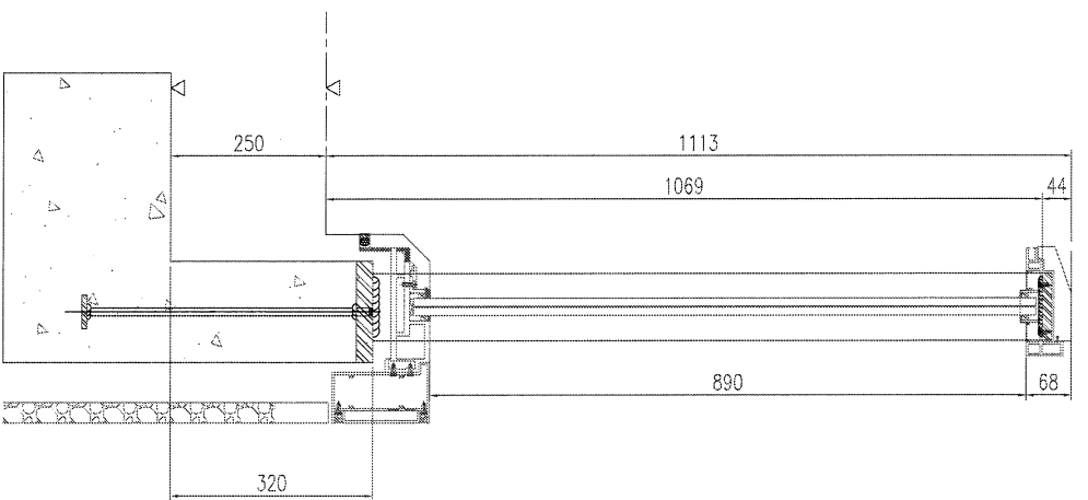
21 SECTION DETAIL 5:1
