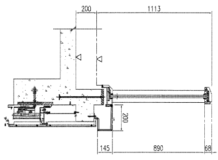
2-1 SECTION DETAIL
