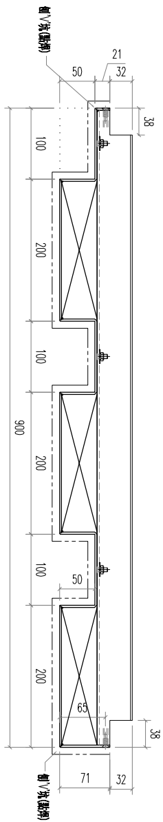
SECTION B-B
