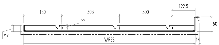
SECTION A1-A1
