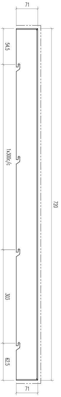
SECTION C-C
