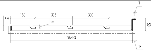
SECTION A1-A1
