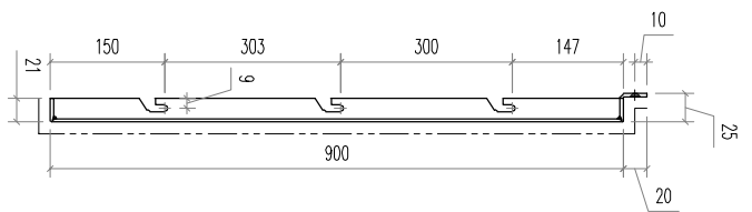
SECTION A1-A1
