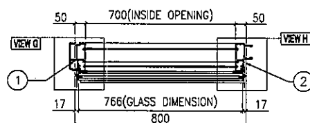
SECTION C-C
