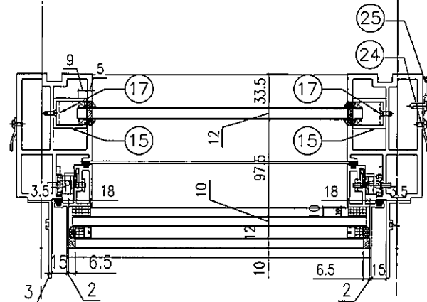
VIEW C
