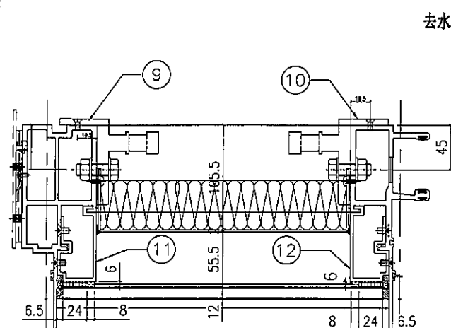
VIEW A
