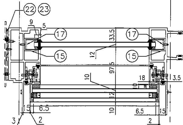
VIEW C
