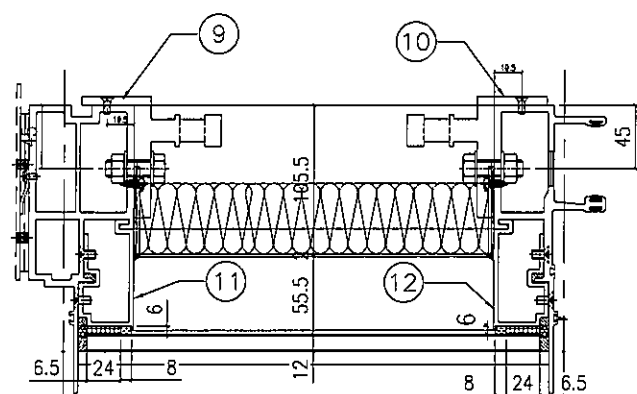
VIEW A
