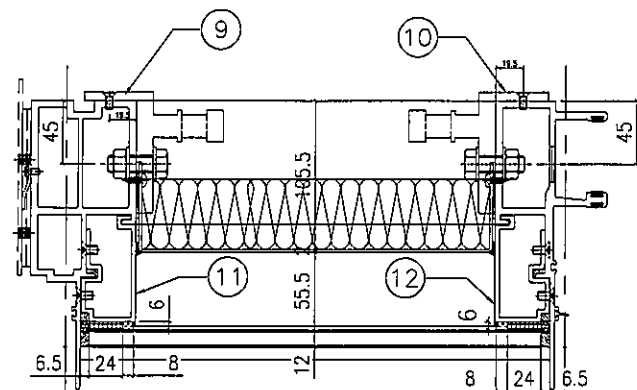
VIEW A
