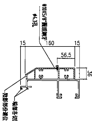
SECTION B-B
