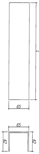
鋁折件2/20/21/22/23
