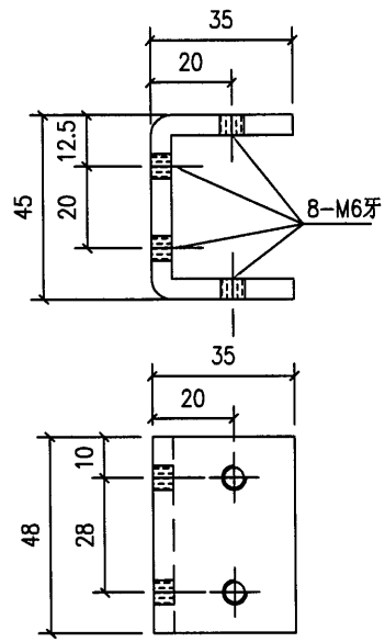
J853-M1-2 數量:60个
