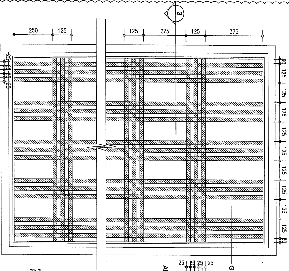
1 ALUMINIUM CLADDING CUTOUT CHINESE PATTERN DETAIL 02 HOUSE A (TYPE F)
