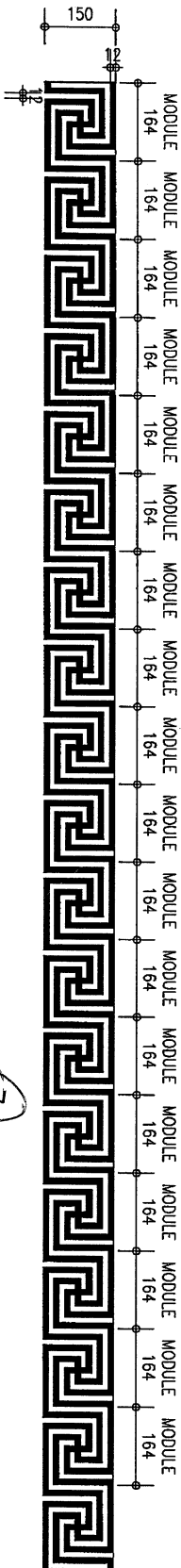
3 ALUMINIUM CLADDING CUTOUT CHINESE PATTERN DETAIL 03
