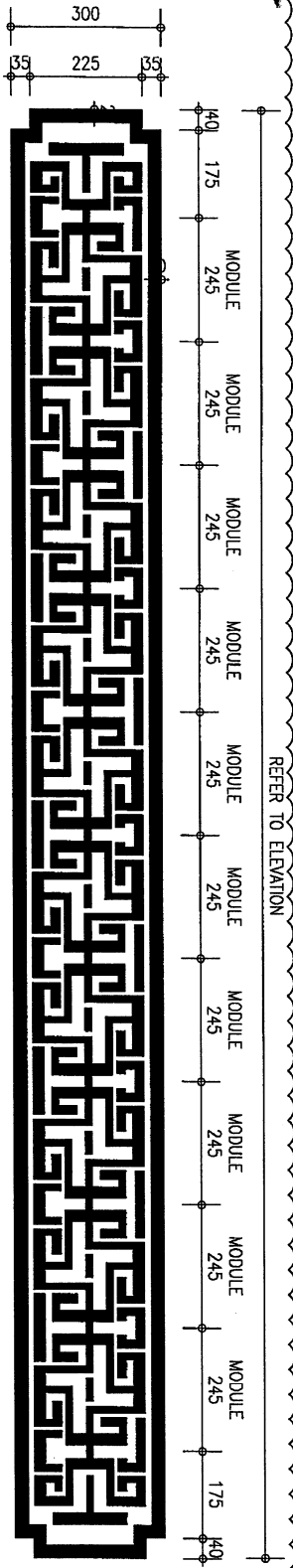
1 ALUMINIUM CLADDING CUTOUT CHINESE PATTERN DETAIL 02 HOUSE A (TYPE F)
