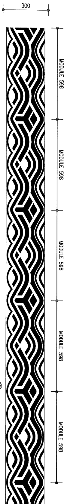
1 ALUMINIUM CLADDING CUTOUT CHINESE PATTERN DETAIL 01
