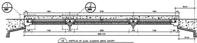
1B PARTPLAN OF ALUM. CLADDING ABOVE CANOPY 4045 FOR AL-504-804.70(4)(L2,L3,L4,Y)
