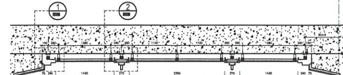
1C PARTPLAN OF ALUM. CLADDING ABOVE CANOPY 4045 FOR AL-504-804.70(4)(L2,L3,L4,Y)
