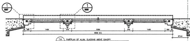
1A PARTPLAN OF ALUM. CLADDING ABOVE CANOPY 4045 FOR AL-504-804.70(4)(L2,L3,L4,Y)
