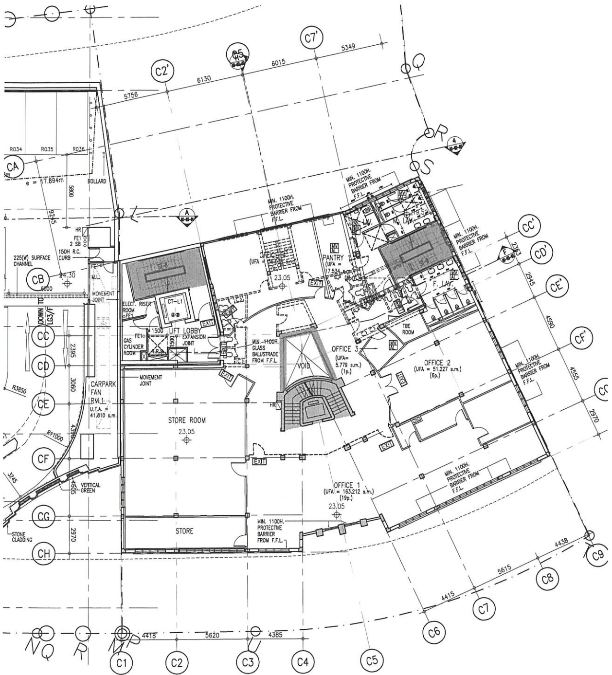
CLOCK TOWER BUILDING SECOND FLOOR PLAN
