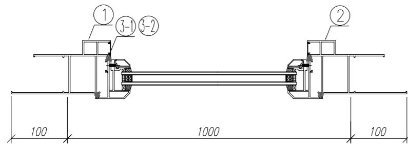
剖-C
