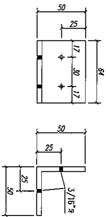
50*50*5角碼L=64MM
