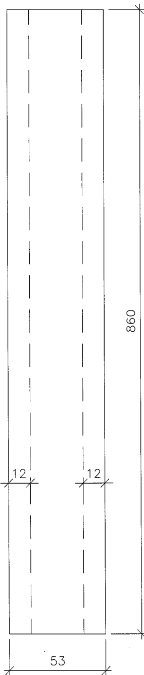
VIEW A
