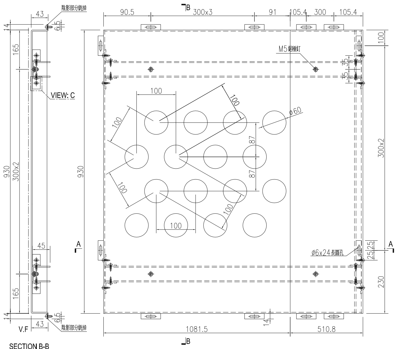
SECTION B-B
