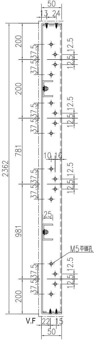
SECTION B-B
