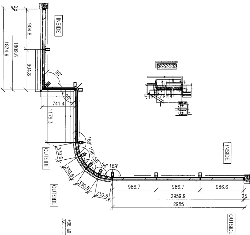
PARTIAL PLAN
