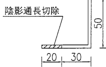
50x50x3鋁角 ME0001961
