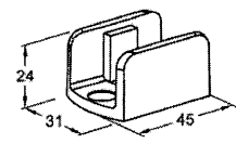
UG-5ADJ Stainless Steel Single U (for 13.52, 15, 15.52, 17.52, 19, 19.52 & 21.52 mm Glass Thickness)
