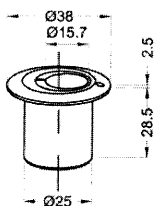
9002 - Eccentric Bolt Keeper
