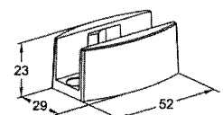
UG-ALT4 Stainless Steel Single U Floor Guide (for 8, 10, 12 & 13.52 mm Glass Thickness)
