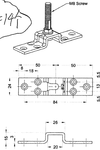
MH85 Stainless Steel Bracket
