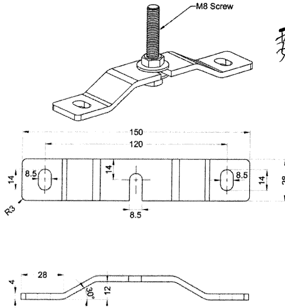
MH120 Plated Steel Bracket
