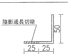
50x50x3鋁角 ME0001961
