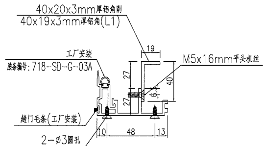
SECTION C-C
