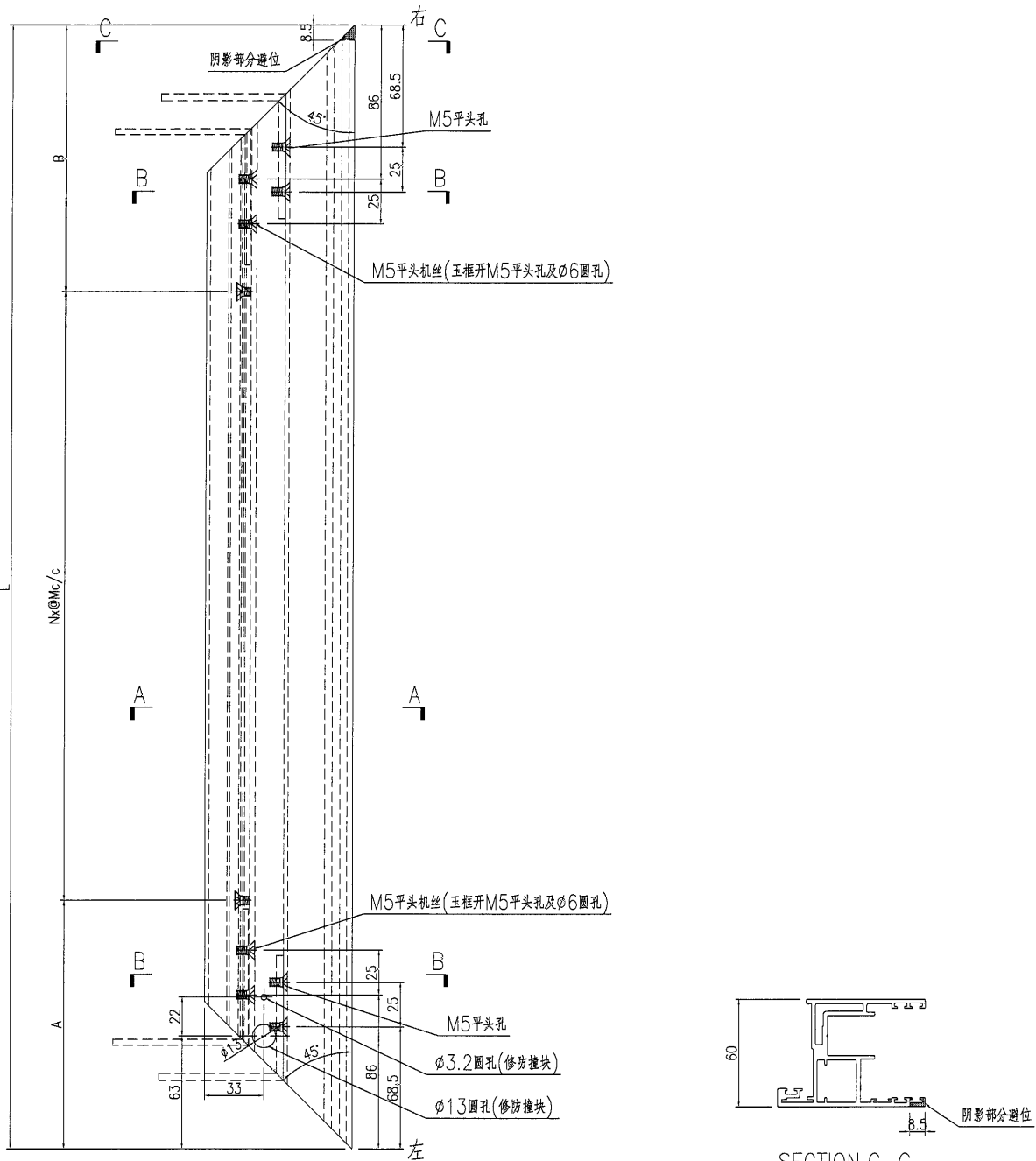
SECTION C-C
