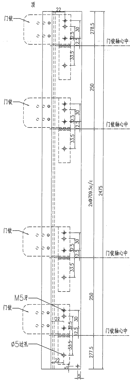
VIEW B-B
