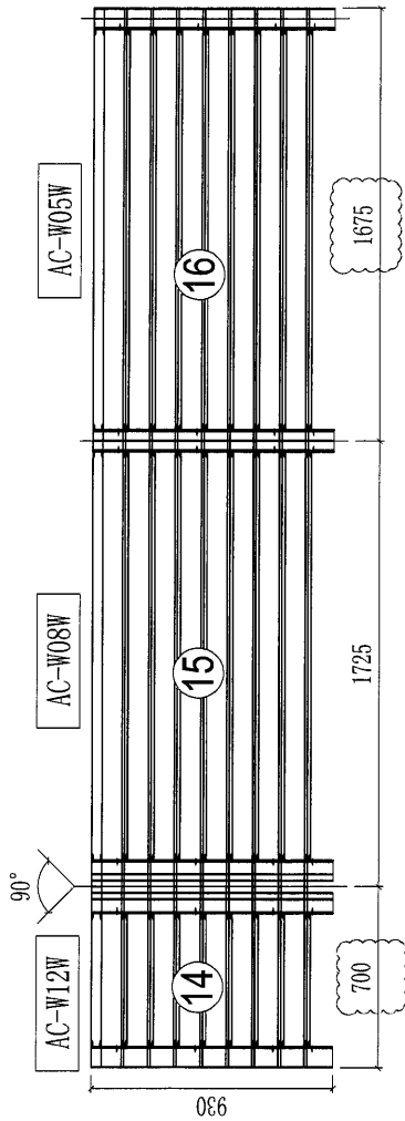
ELEVATION (AC25) T1/E/1F&T2/E/1F
