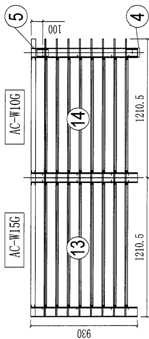
○ ELEVATION (AC10a) T2A/B/1F
