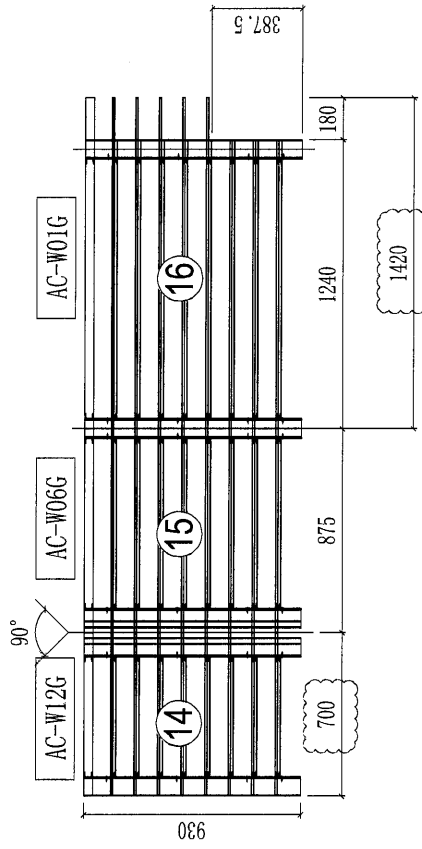
ELEVATION (AC10b) T1A/C/1F
