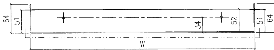
SECTION B-B
