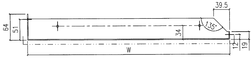
SECTION B-B
