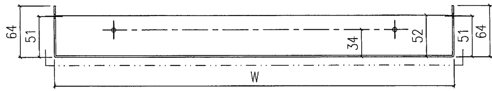
SECTION B-B
