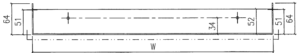
SECTION B-B
