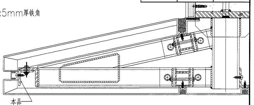
4a TYPICAL DETAIL OF ALUMINIUM FEATURE (AL2-1) D01 SCALE: 1 : 3
