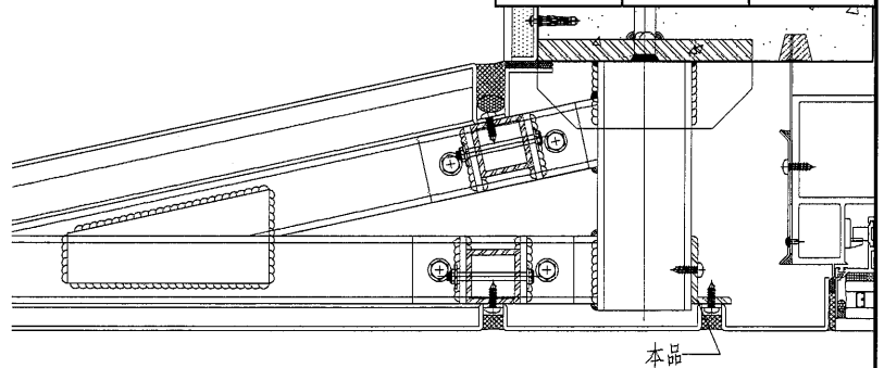
4a TYPICAL DETAIL OF ALUMINIUM FEATURE (AL2-1) D01 SCALE: 1 : 3
