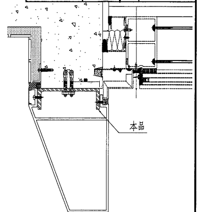
3 D10 TYPICAL DETAIL OF ALUMINIUM FEATURE (AL3b) SCALE: 1 : 3
