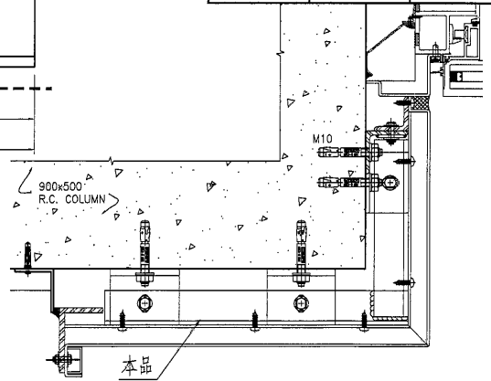
② PLAN DETAIL OF ALUMINIUM CLADDING (AL4) D02 SCALE: 1 : 3
