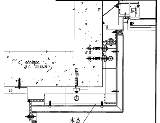
PLAN DETAIL OF ALUMINIUM CLADDING (AL4a)
