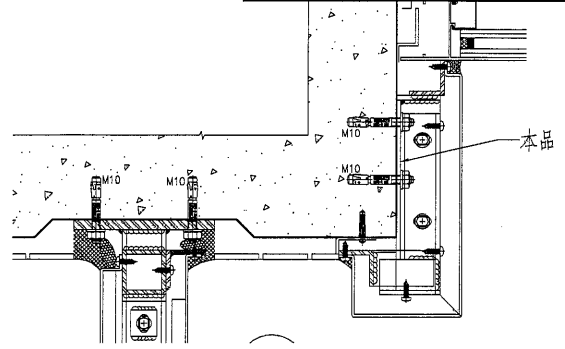
2 DETAIL OF ALUMINIUM CLADDING (AL10-1) D07 SCALE: 1 : 2
