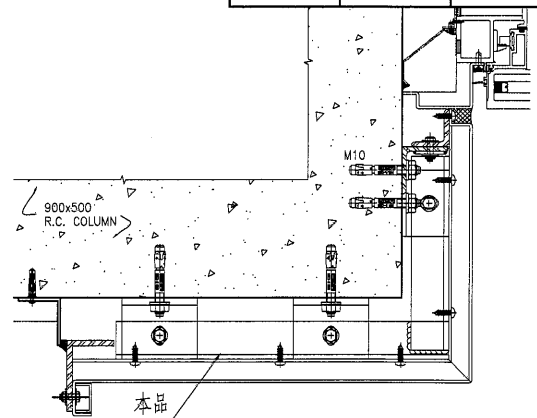
PLAN DETAIL OF ALUMINIUM CLADDING (AL4)
