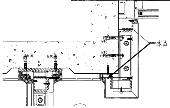
2 DETAIL OF ALUMINIUM CLADDING (AL10-1) SCALE: 1 : 3
