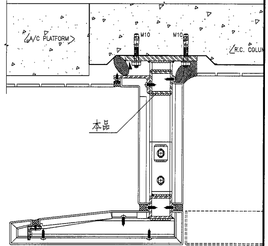
2 508 SCALE: 1 : 3 DETAIL OF ALUMINIUM CLADDING (AL10) AL10-1
