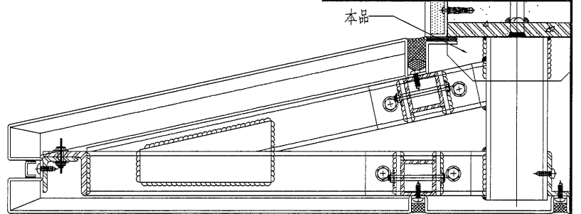
4a D01 TYPICAL DETAIL OF ALUMINIUM FEATURE (AL2-1) SCALE: 1 : 3
