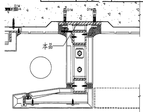
2 D07 SCALE: 1 : 3 DETAIL OF ALUMINIUM CLADDING (AL10)
