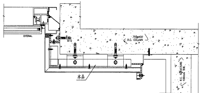
PLAN DETAIL OF ALUMINIUM CLADDING (AL4-1) (FOR 1/F-32/F HOR. JOINT) SCALE: 1:3
