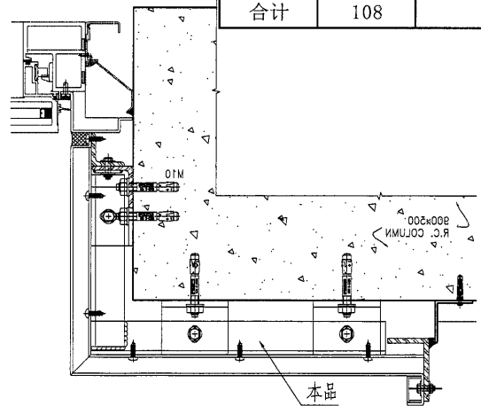
2 PLAN DETAIL OF ALUMINIUM CLADDING (AL4) D02 SCALE: 1 : 3
