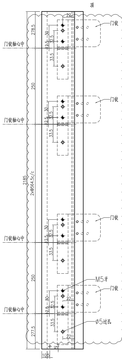
VIEW B-B
