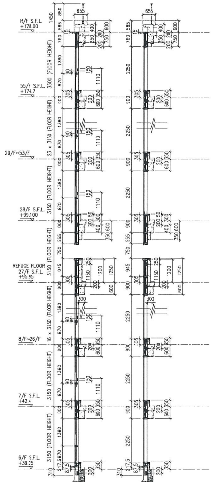
2 TYPICAL SECTION FOR CURTAIN WALL
