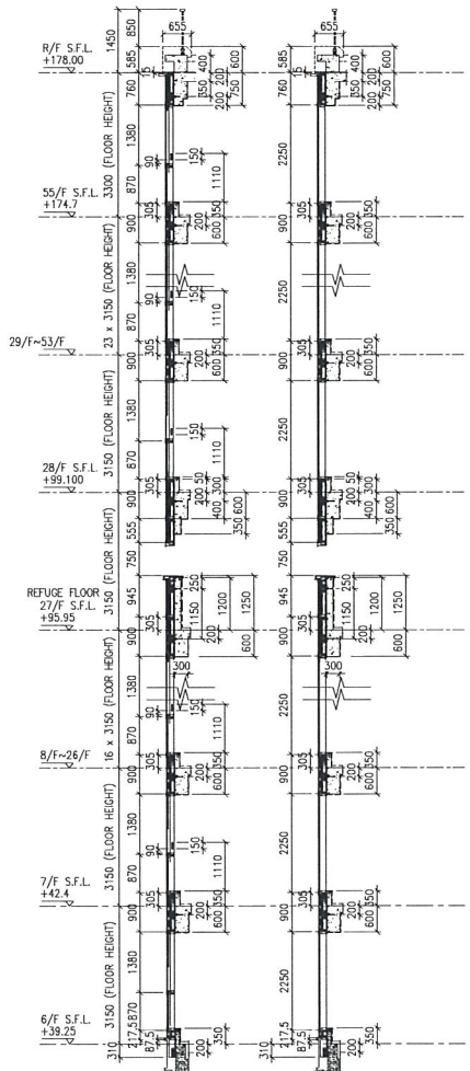
(2) TYPICAL SECTION FOR CURTAIN WALL (3) TYPICAL SECTION FOR CURTAIN WALL
