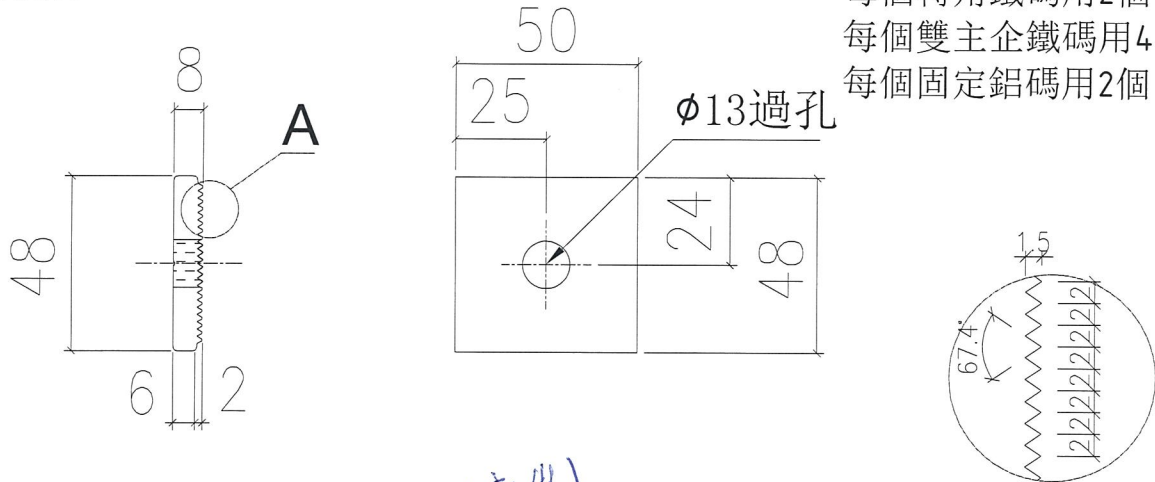
A SCALE 3:1
