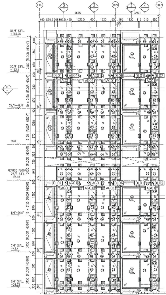
1 PART ELEVATION FOR CURTAIN WALL
