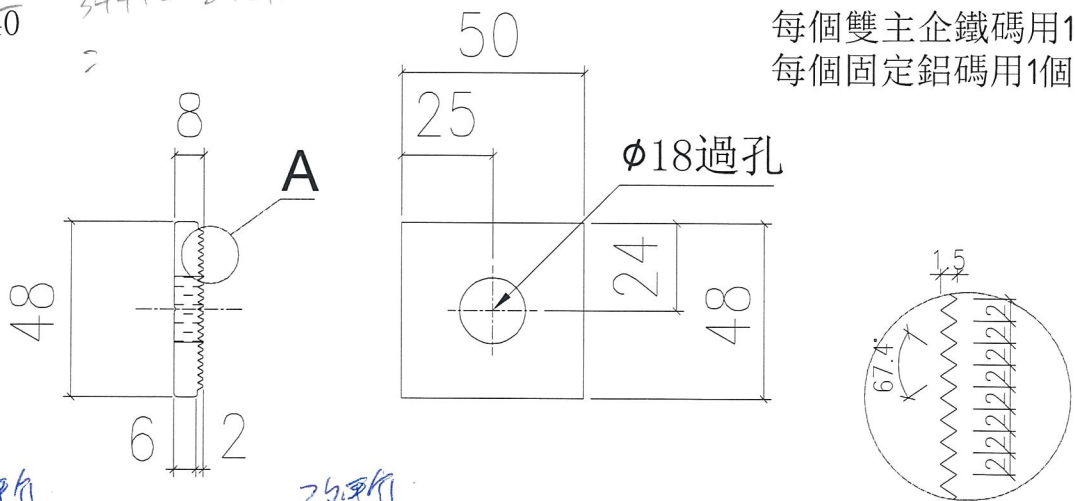
A SCALE 3:1
