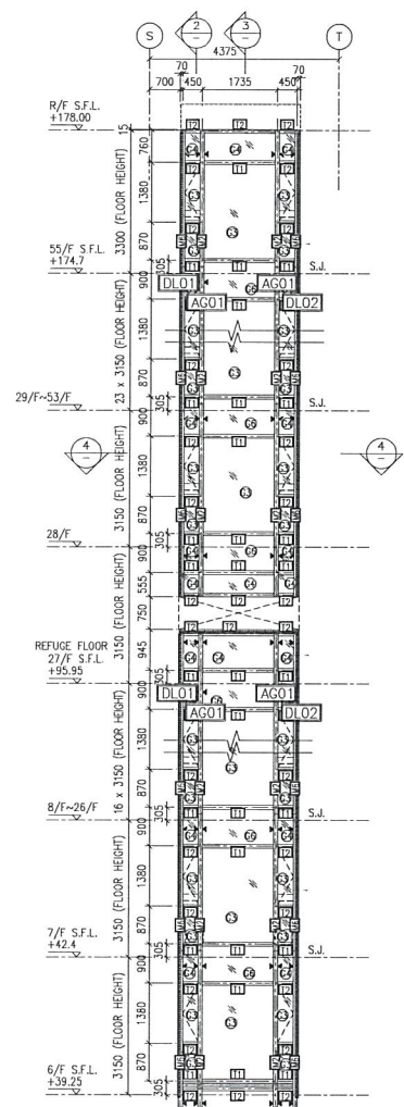
1 PART ELEVATION FOR CURTAIN WALL
