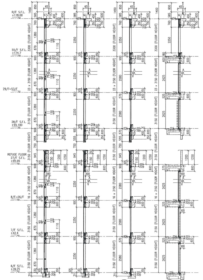
2 TYPICAL SECTION FOR CURTAIN WALL
