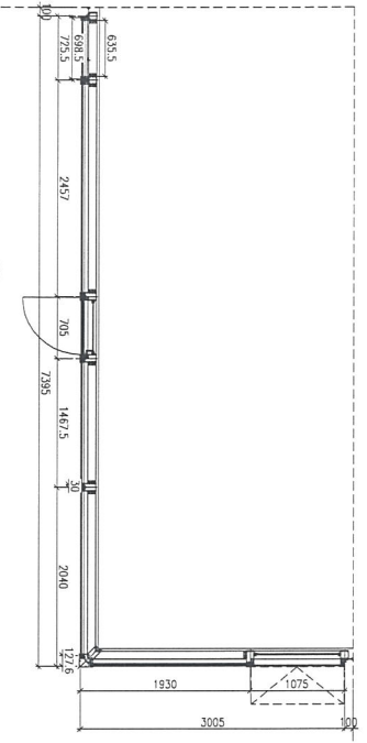
4 PLAN FOR CURTAIN WALL
