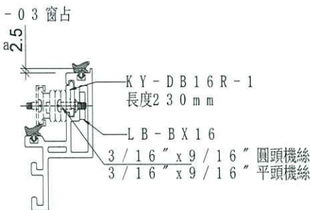
SECION: B-B
