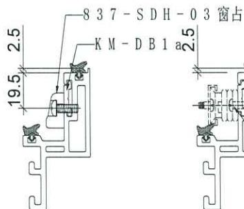
SECION: C-C
