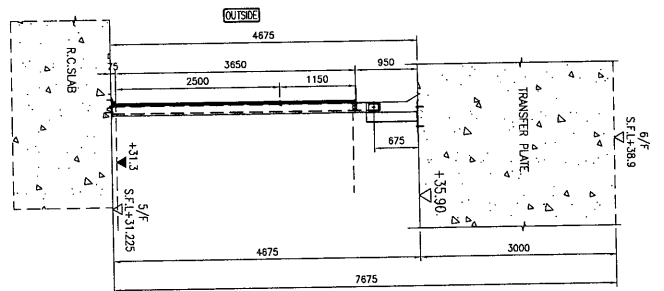
4-4 SECTION OF WINDOW UNIT
