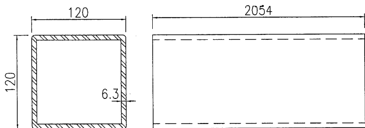
120x120x6.3mm厚鐵通(熱浸)
