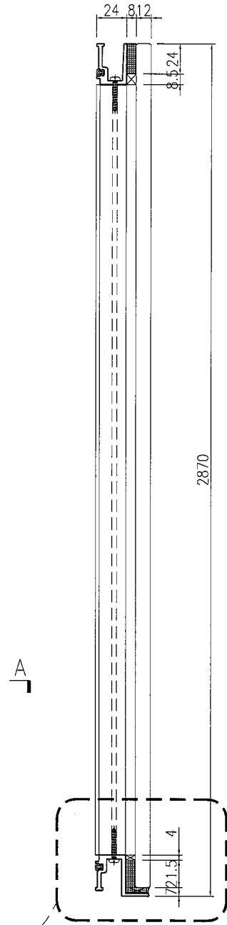
SECTION B-B
