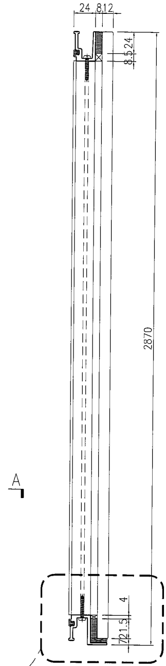
SECTION B-B
