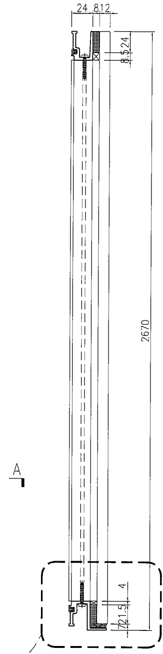
SECTION B-B
