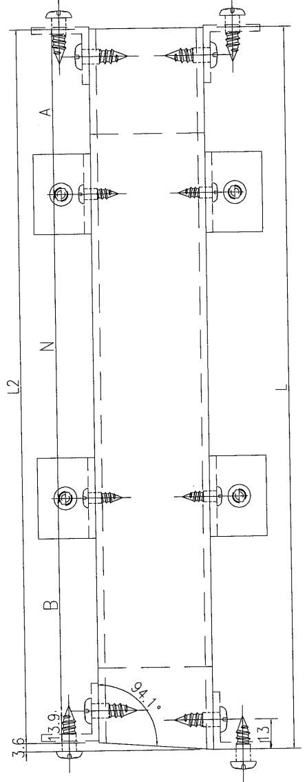
剖圖C-C
