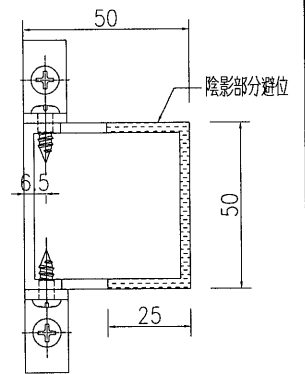
剖圖D-D
