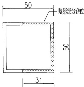
剖圖C-C
