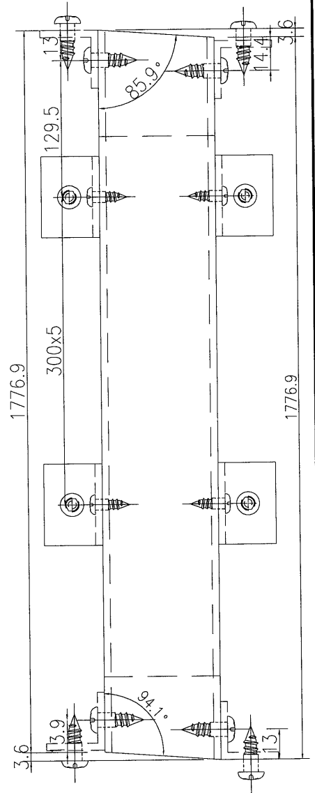
剖圖C-C
