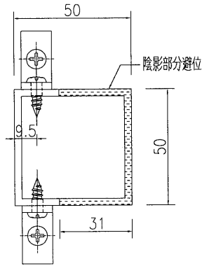
剖圖D-D
