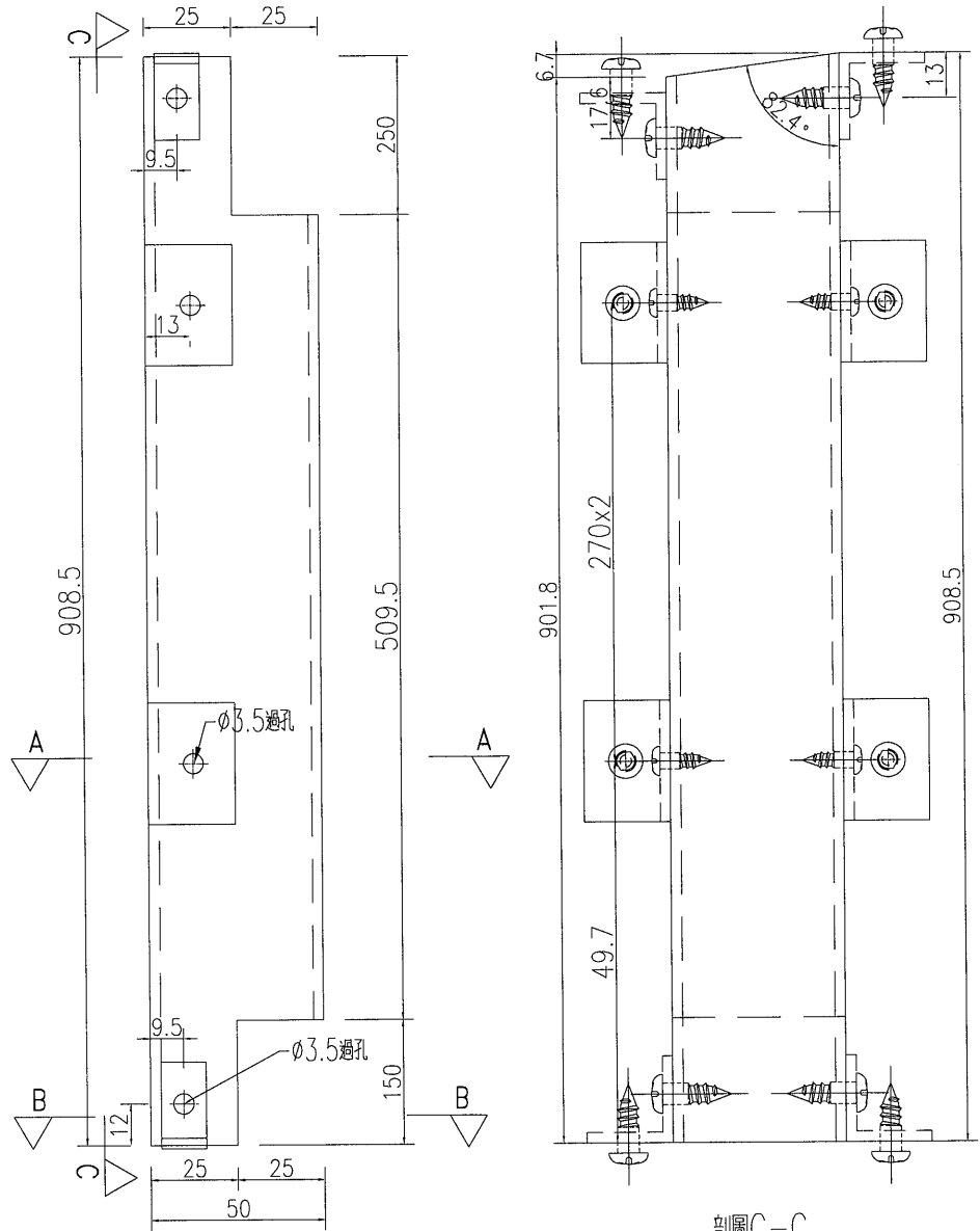
剖圖C-C
