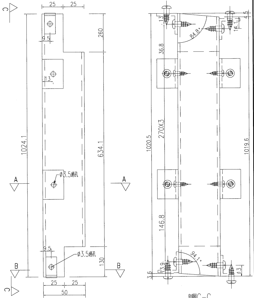
剖圖C-C
