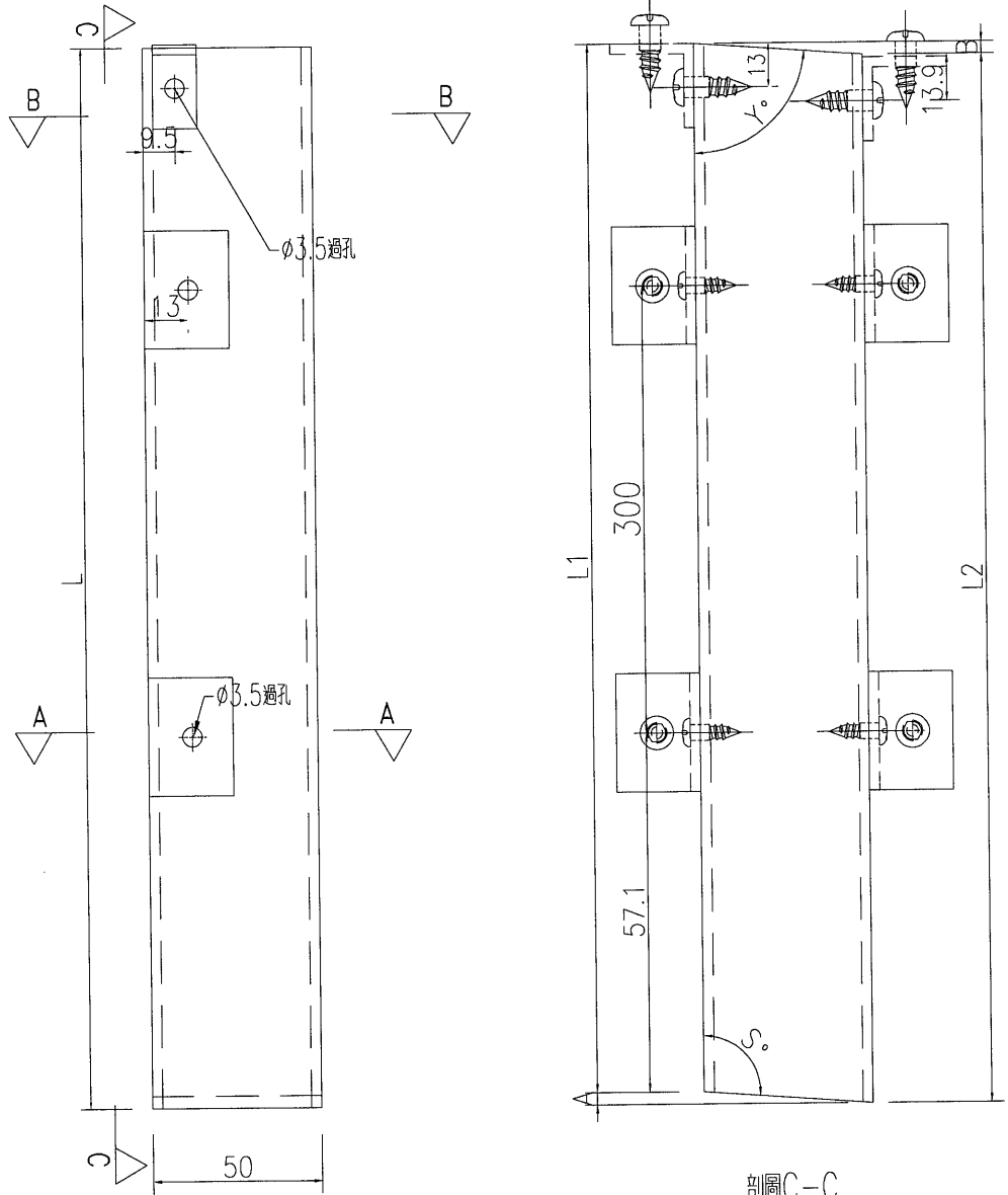
剖圖C-C
