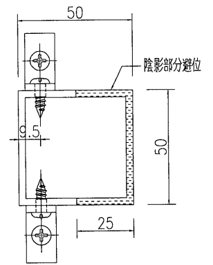
剖圖D-D
