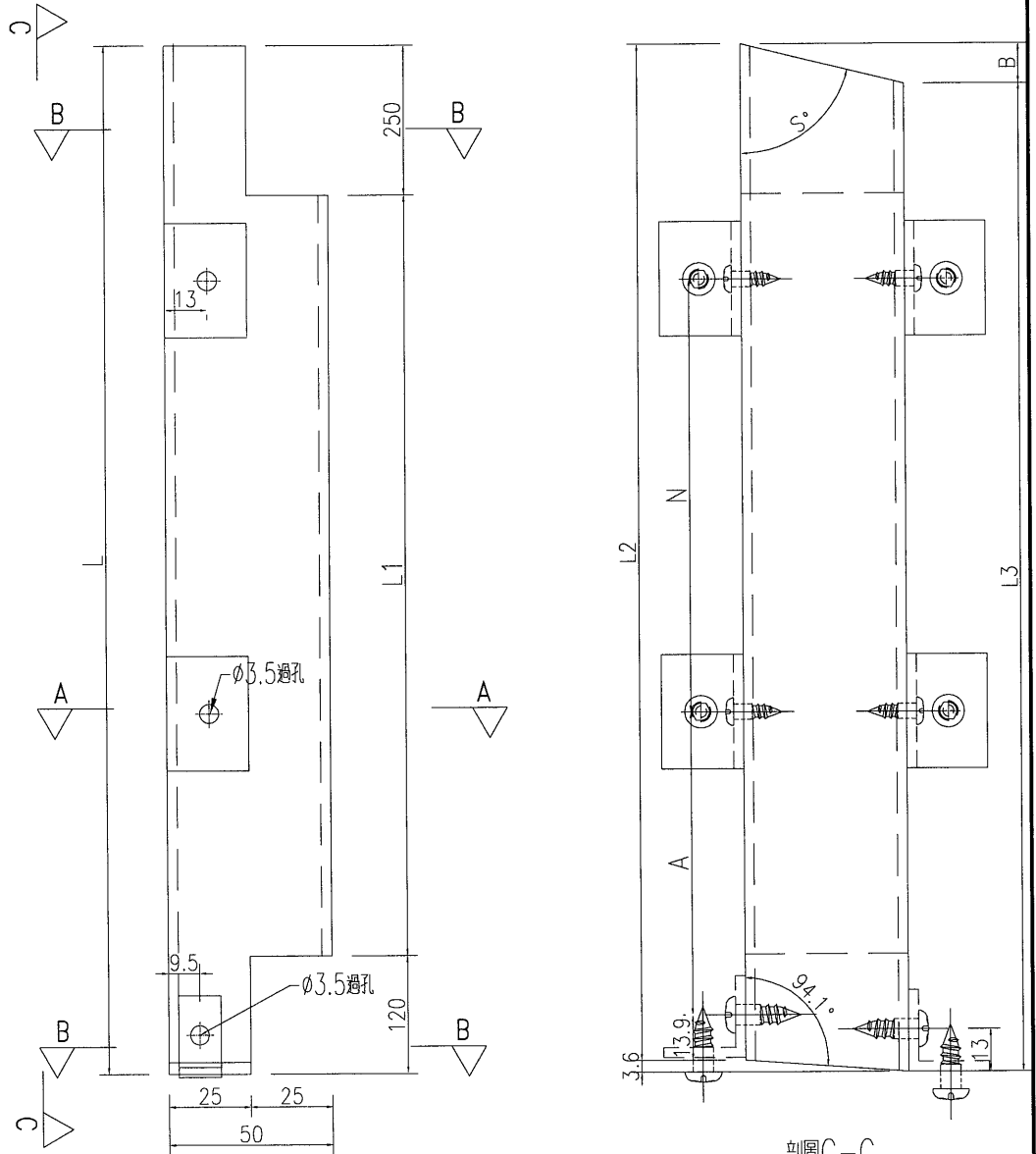
剖圖C-C
