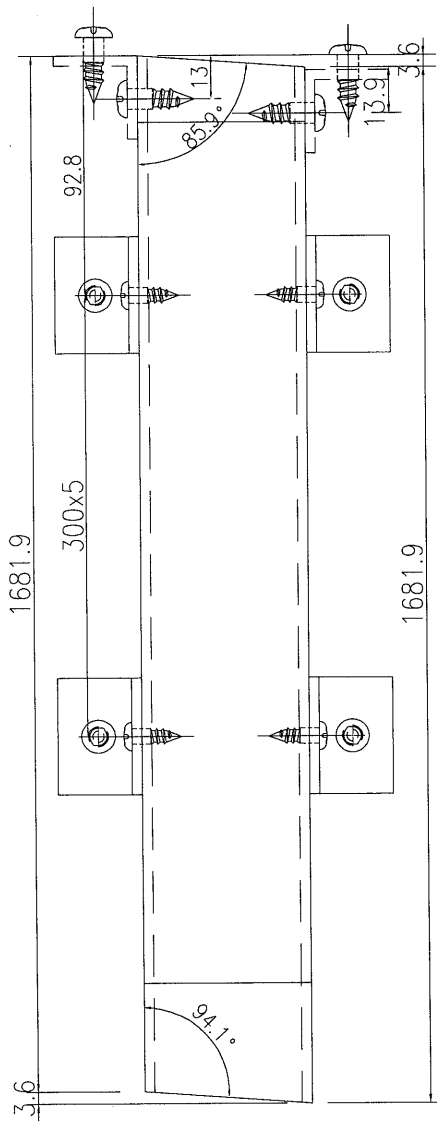
剖圖C-C
