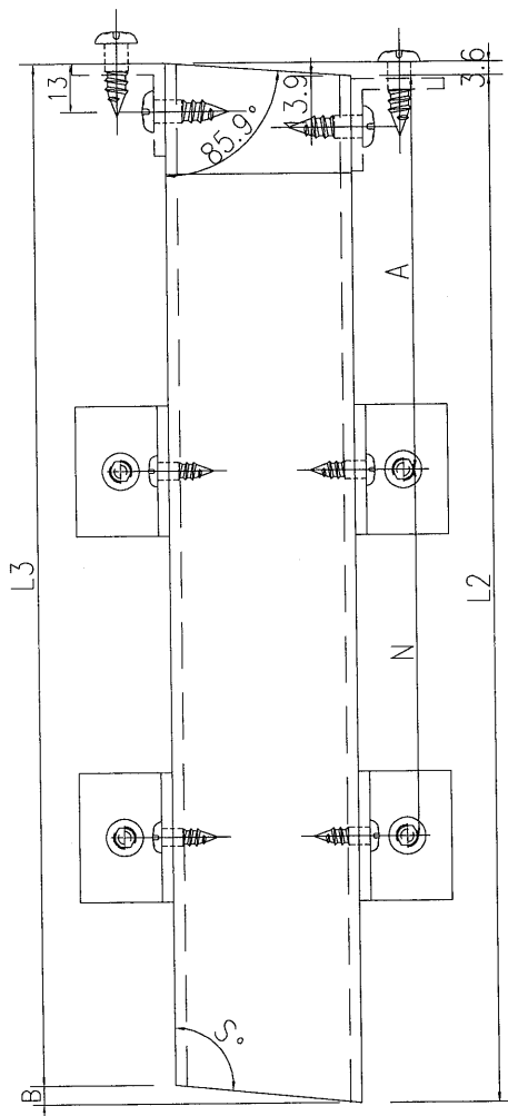
剖圖C-C
