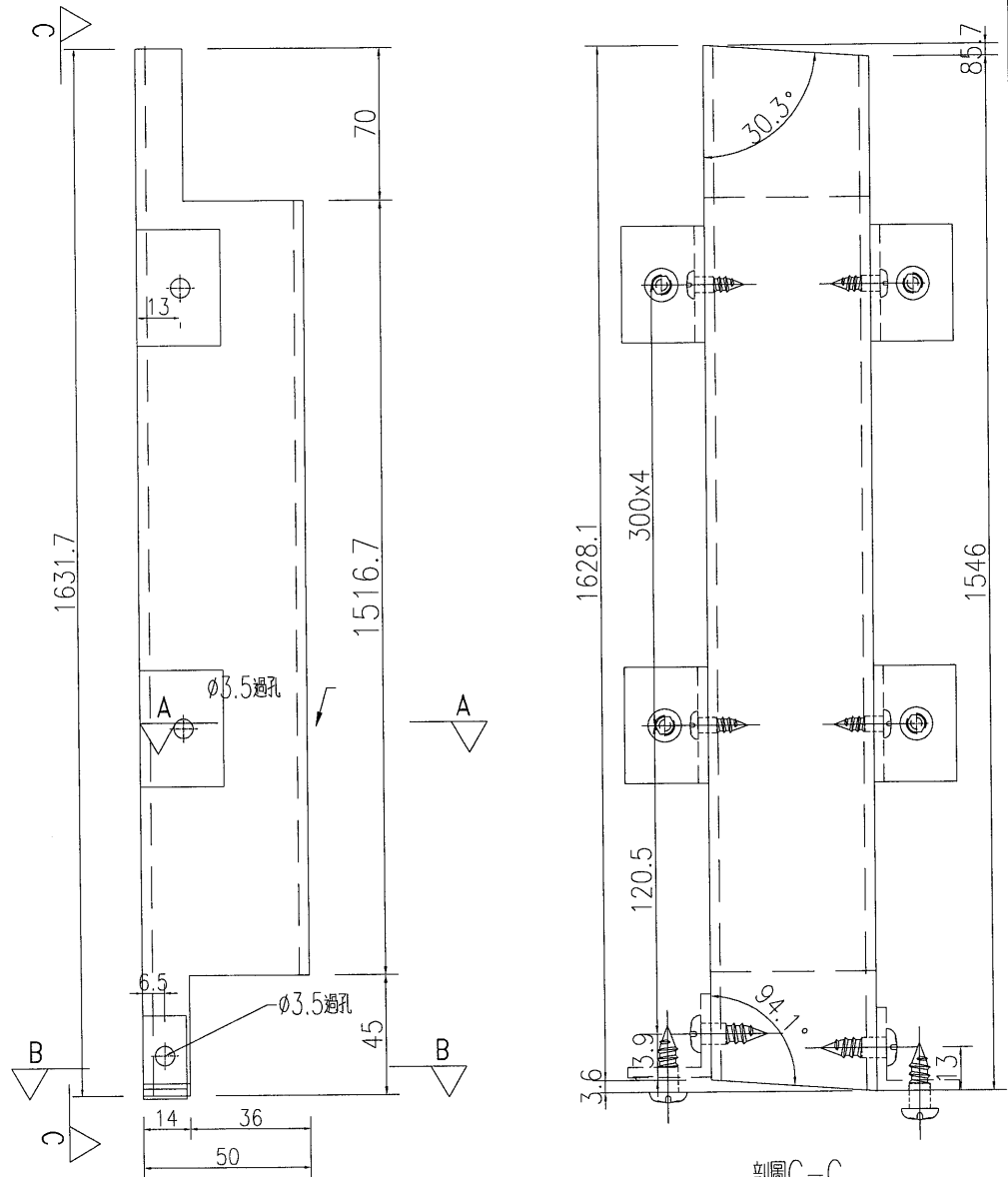
剖圖C-C
