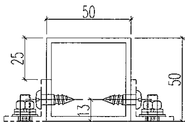
剖圖C-C
