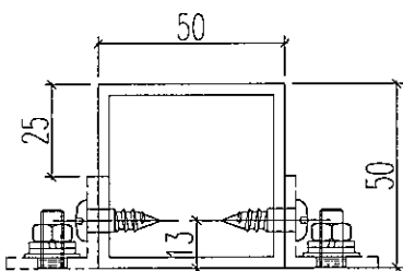
剖圖C-C
