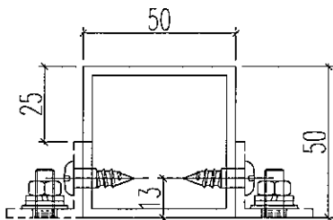
剖圖C-C
