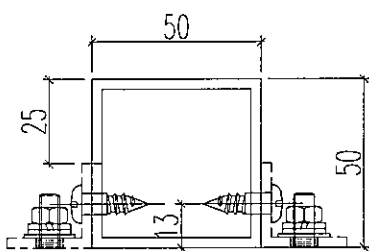
剖圖C-C
