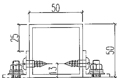
剖圖C-C
