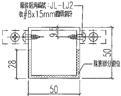
剖圖C-C
