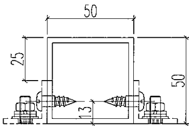
剖圖C-C
