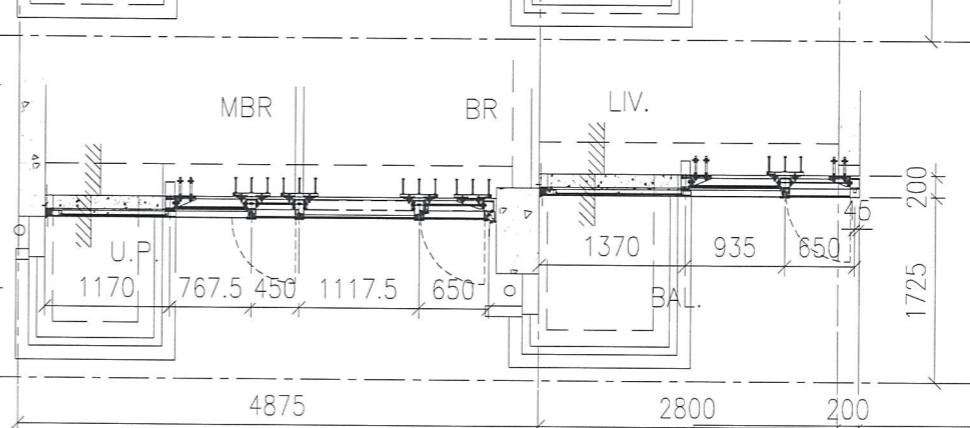
6 PART PLAN FOR CURTAIN WALL
