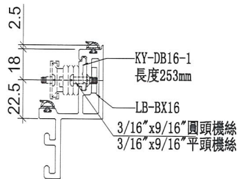
SECION: B-B
