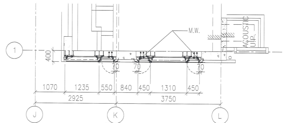
4 - PART PLAN FOR CURTAIN WALL
