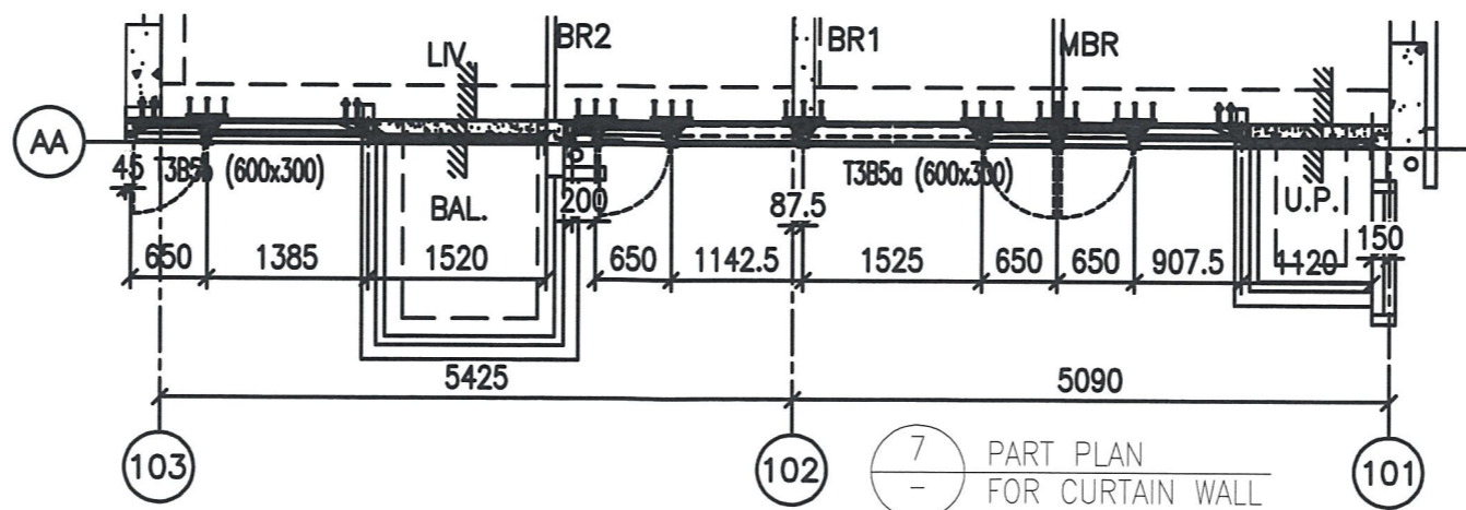
6 PART PLAN FOR CURTAIN WALL
