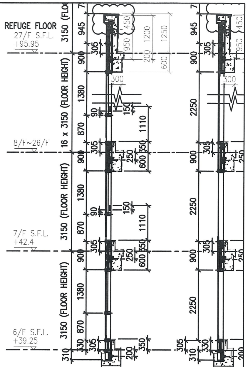
2 TYPICAL SECTION FOR CURTAIN WALL
