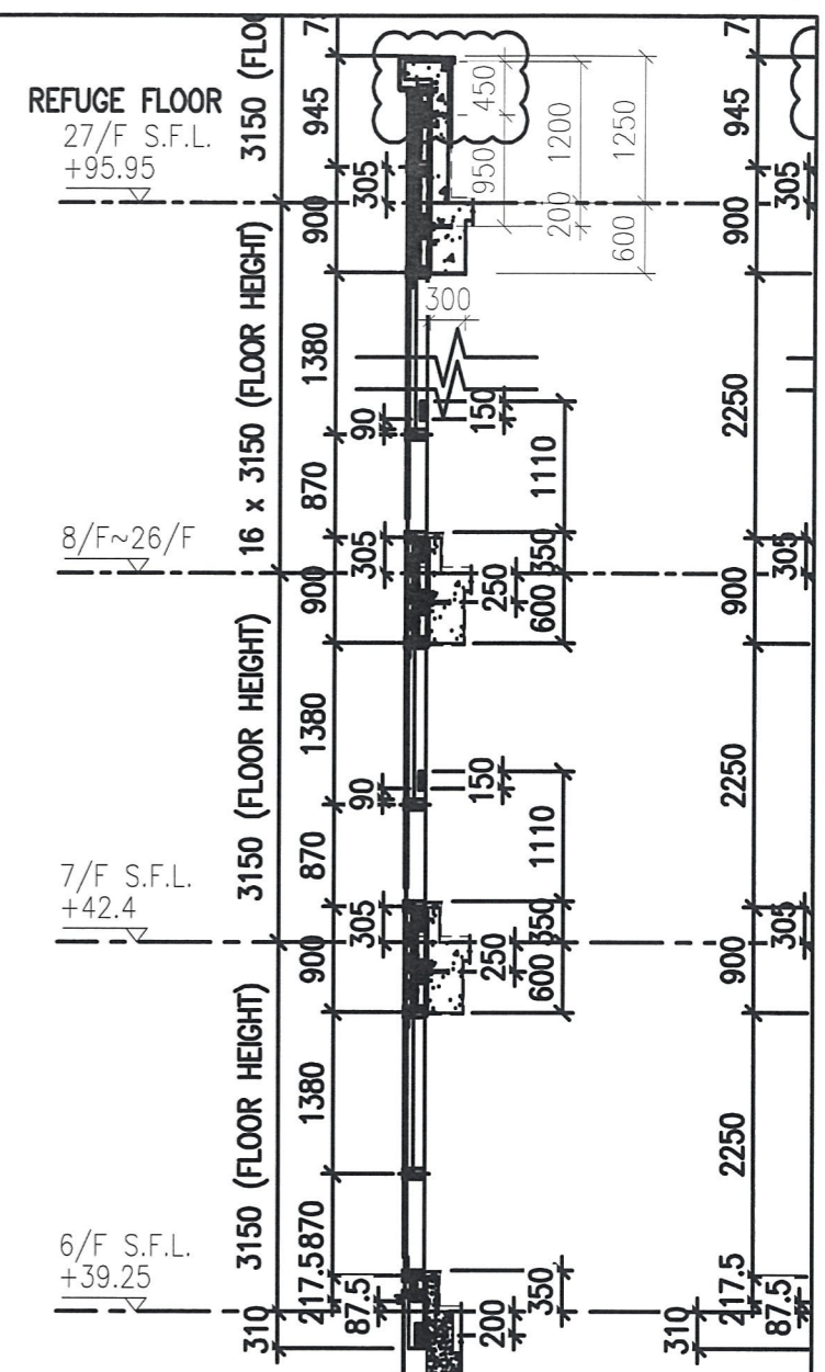
2 TYPICAL SECTION FOR CURTAIN WALL
